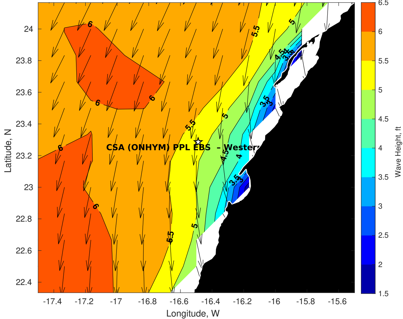
Wave Height (ft) for CSA (ONHYM) PPL EBS - Western Sahara at 28-Jul-2025 09:00:00
