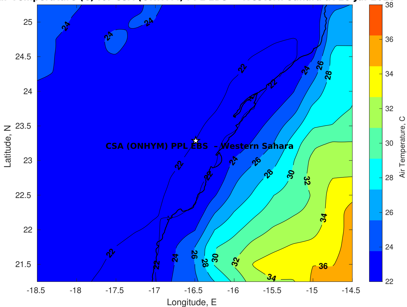
Air Temperature (C) for CSA (ONHYM) PPL EBS - Western Sahara at 28-Jul-2025
