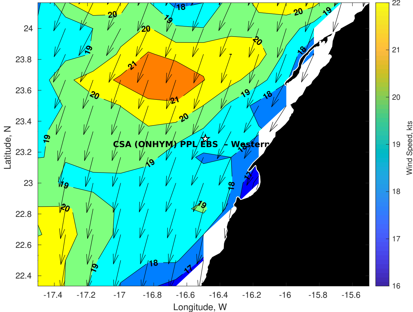
Winds (kts) for CSA (ONHYM) PPL EBS - Western Sahara at 28-Jul-2025 09:00:00
