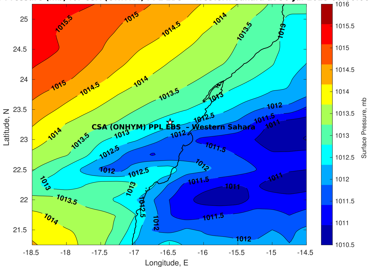
Surface Pressure (mb) for CSA (ONHYM) PPL EBS - Western Sahara at 30-Jul-2025 00:00:00
