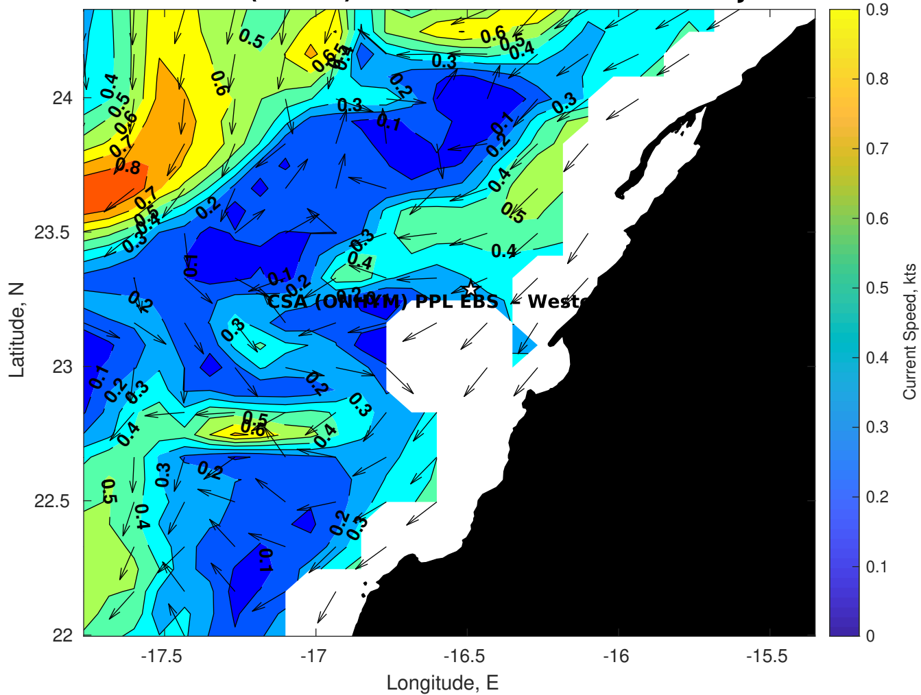
Surface Currents for CSA (ONHYM) PPL EBS - Western Sahara at 25-Jul-2025 00:00:00
