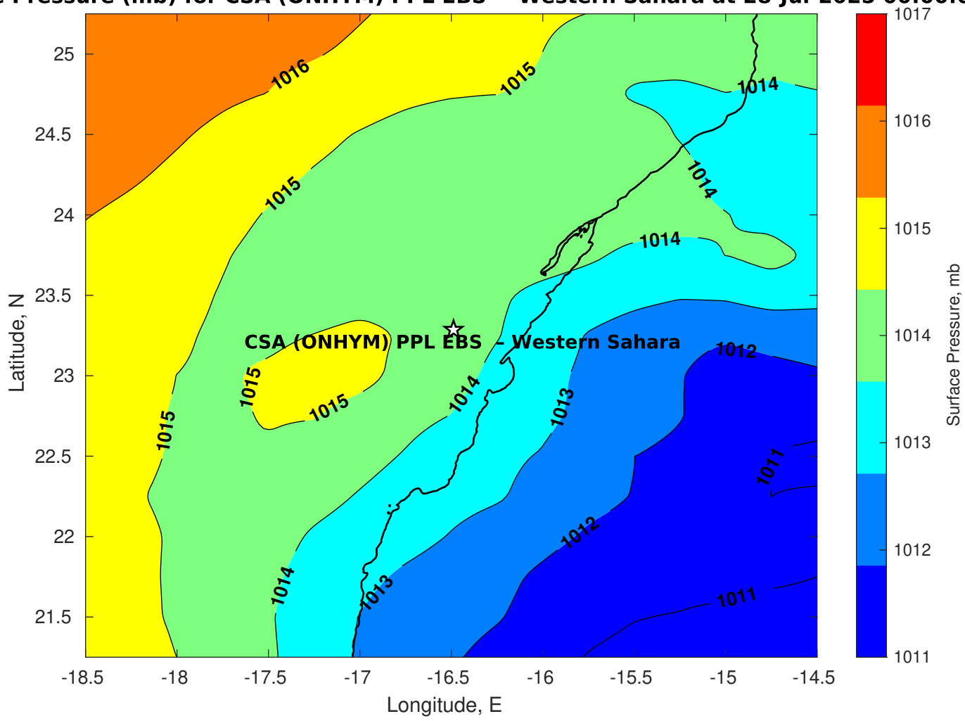
Surface Pressure (mb) for CSA (ONHYM) PPL EBS - Western Sahara at 28-Jul-2025 00:00:00
