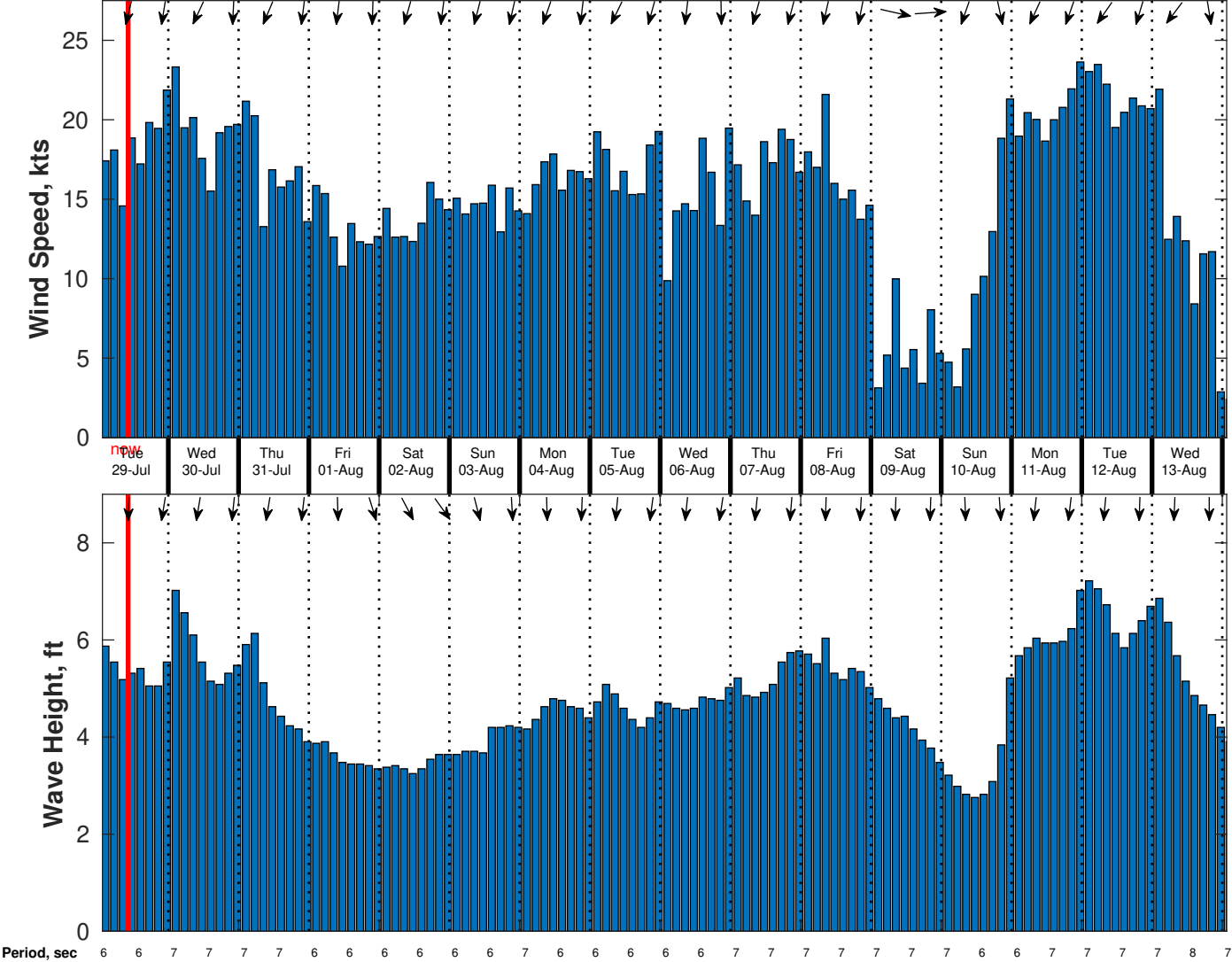
Wind & Wave Forecast for CSA (ONHYM) PPL EBS - Western Sahara from 28-Jul-2025 01:00:00 to 13-Aug-2025 01:00:00
