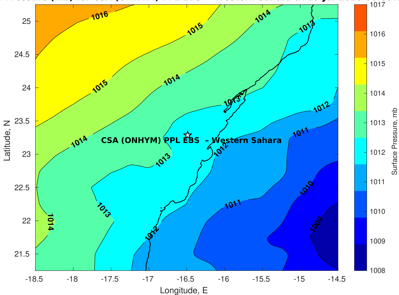
Surface Pressure (mb) for CSA (ONHYM) PPL EBS - Western Sahara at 29-Jul-2025 00:00:00
