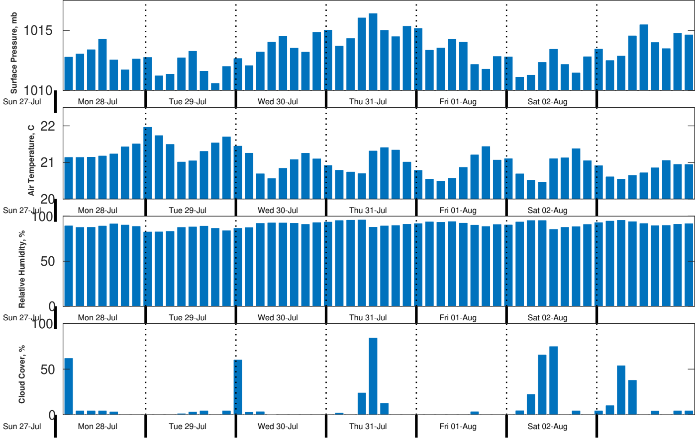
Met Forecast for CSA (ONHYM) PPL EBS - Western Sahara from 28-Jul-2025 00:00:00 to 04-Aug-2025 00:00:00
