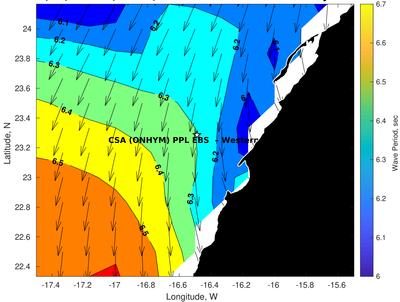
Wave Period (sec) for CSA (ONHYM) PPL EBS - Western Sahara at 28-Jul-2025 09:00:00
