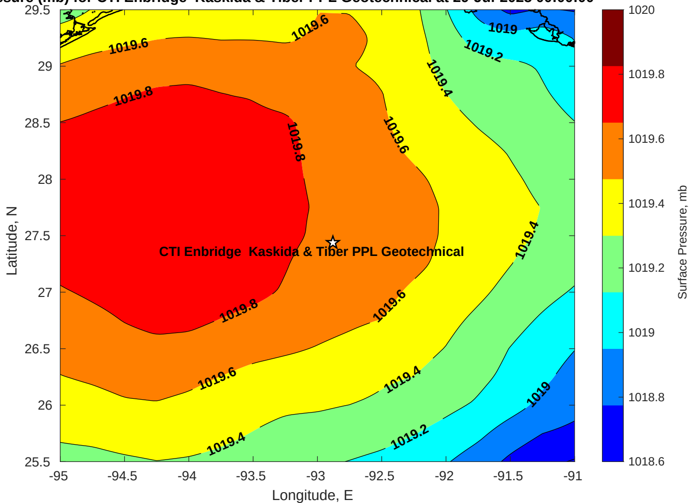
Surface Pressure (mb) for CTI Enbridge Kaskida & Tiber PPL Geotechnical at 29-Jul-2025 00:00:00
