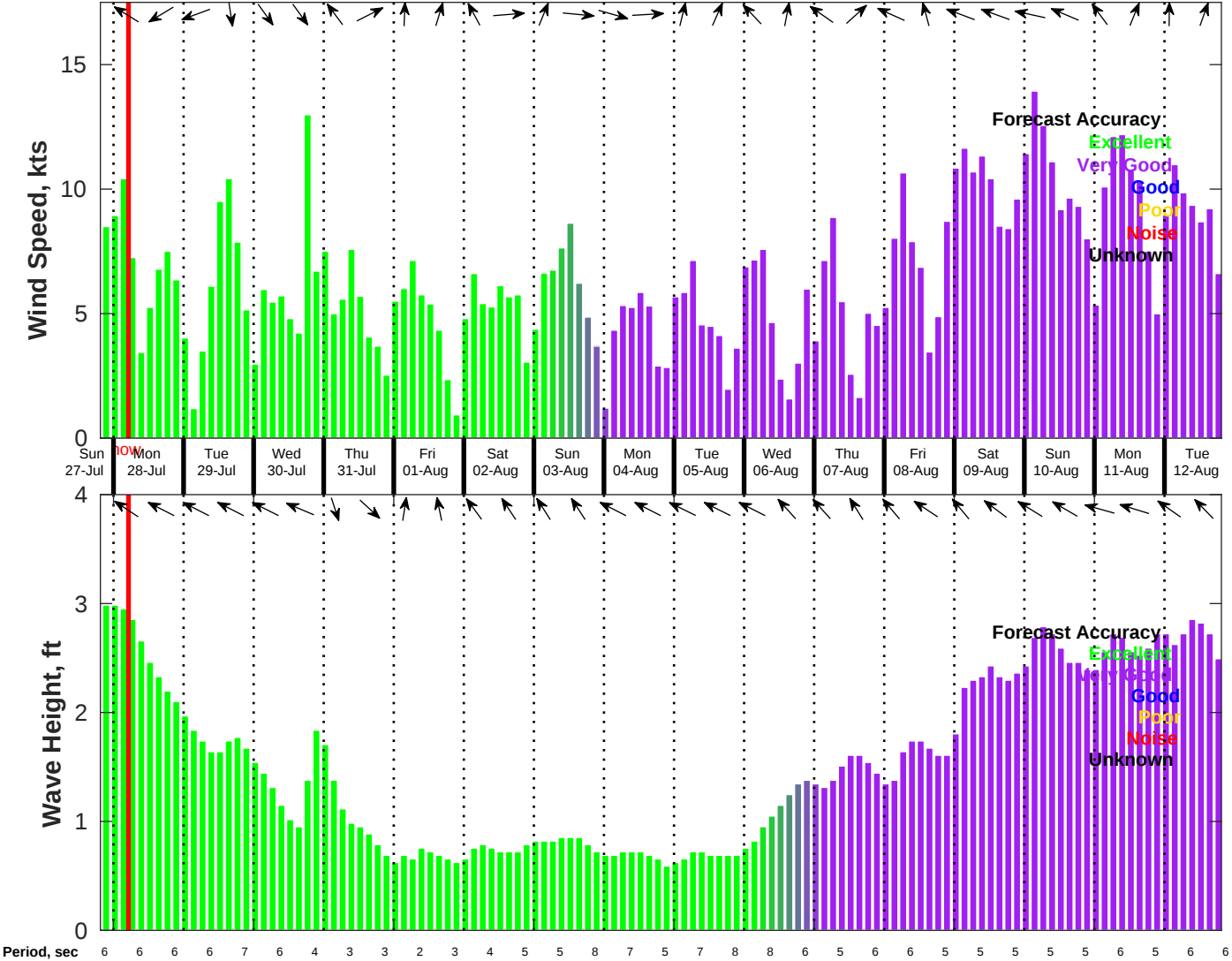
Wind & Wave Forecast for CTI Enbridge Kaskida & Tiber PPL Geotechnical from 27-Jul-2025 20:00:00 to 12-Aug-2025 20:00:00
