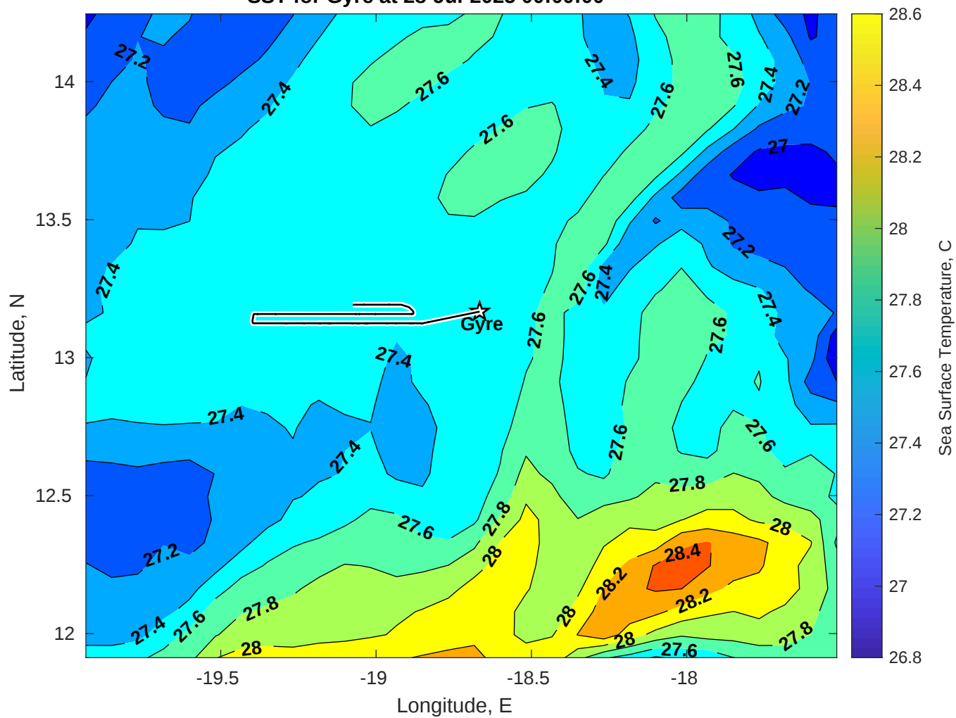
SST for Gyre at 28-Jul-2025 00:00:00
