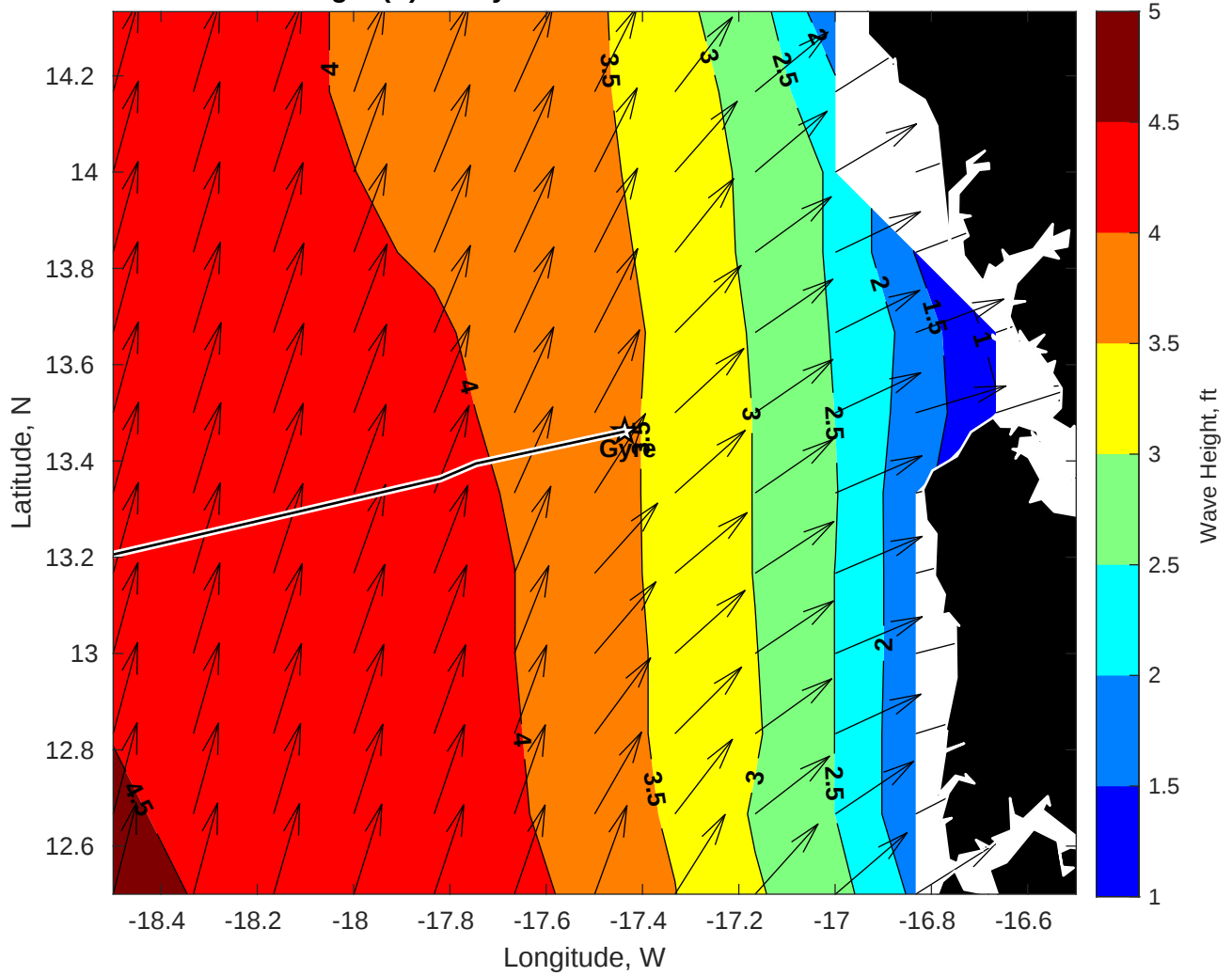
Wave Height (ft) for Gyre at 29-Jul-2025 09:00:00
