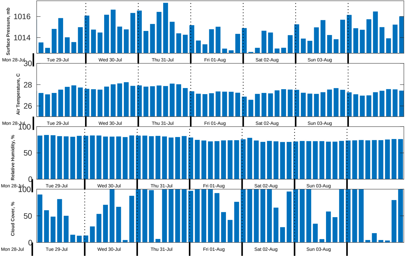
Met Forecast for Gyre from 28-Jul-2025 23:00:00 to 04-Aug-2025 23:00:00
