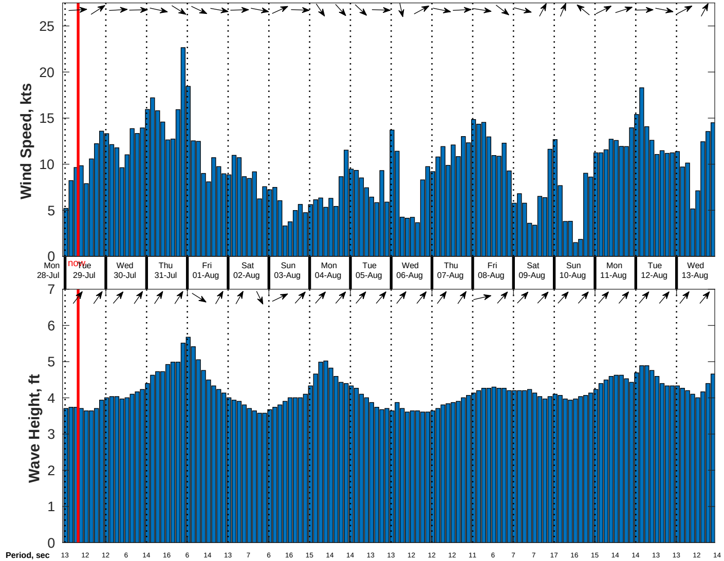
Wind & Wave Forecast for Gyre from 28-Jul-2025 23:00:00 to 13-Aug-2025 23:00:00
