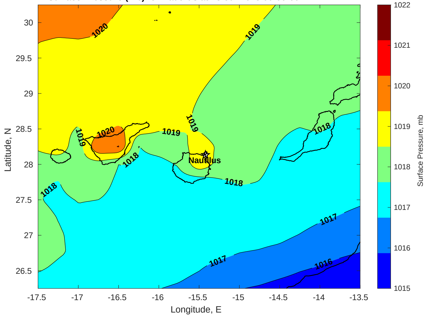
Surface Pressure (mb) for Nautilus at 28-Jul-2025 00:00:00
