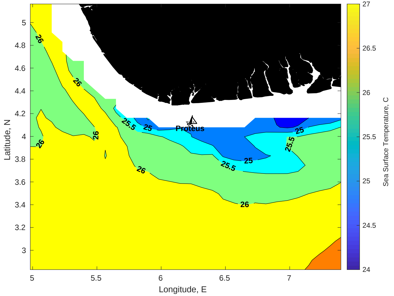
SST for Proteus at 25-Jul-2025 00:00:00
