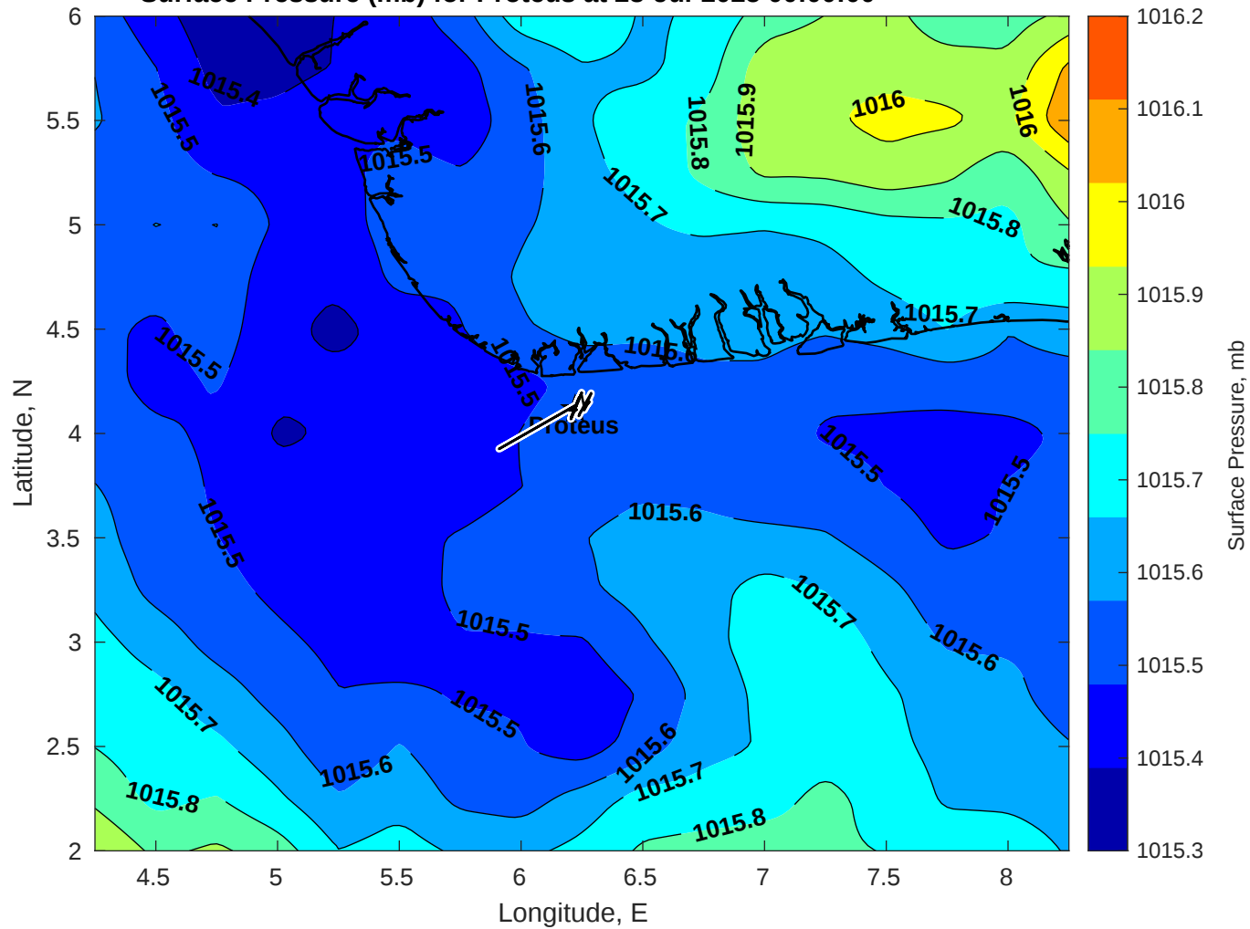
Surface Pressure (mb) for Proteus at 28-Jul-2025 00:00:00
