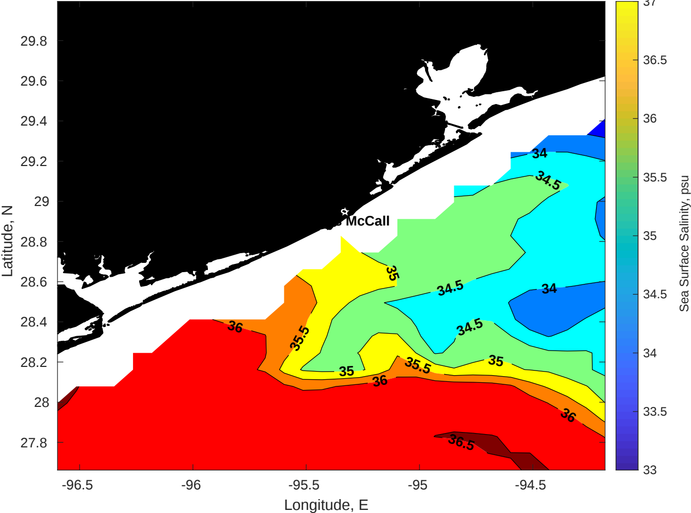
Surface Salinity for Brooks McCall at 28-Jul-2025 00:00:00
