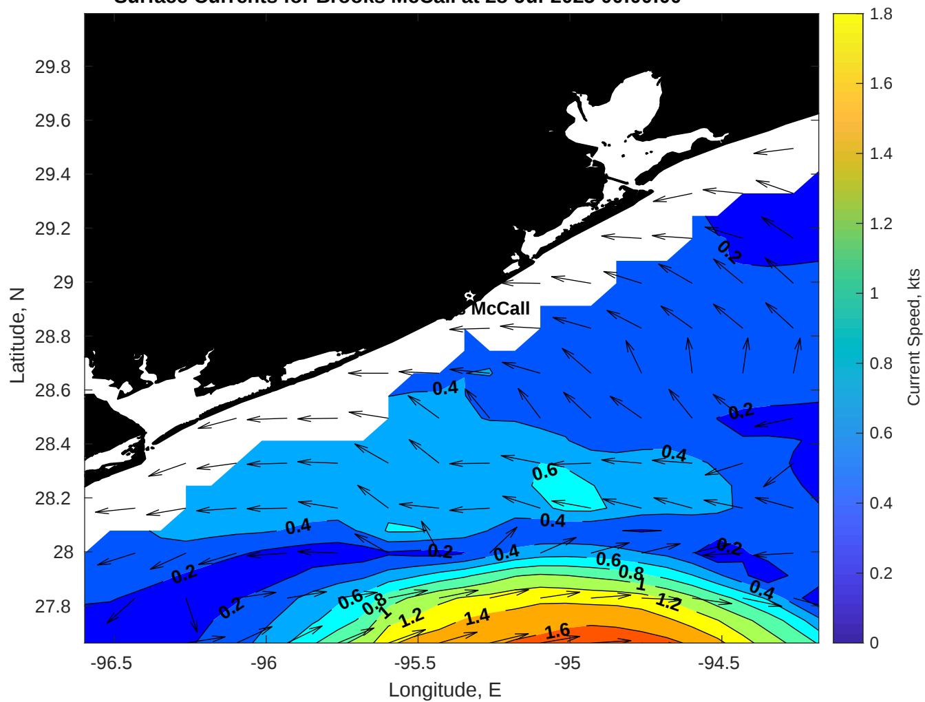
Surface Currents for Brooks McCall at 28-Jul-2025 00:00:00
