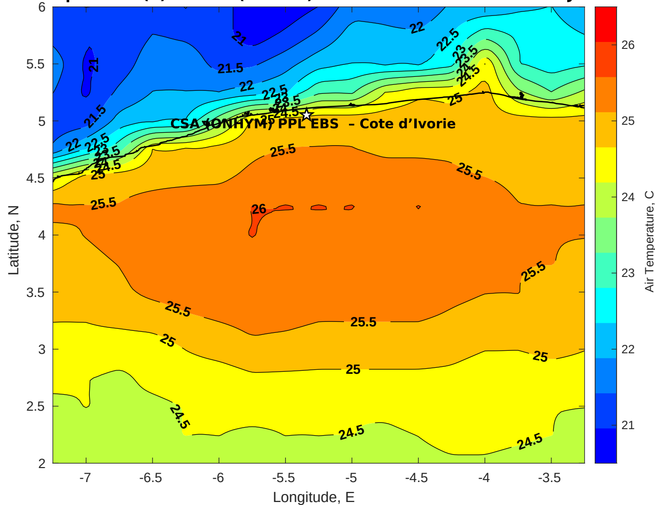
Air Temperature (C) for CSA (ONHYM) PPL EBS - Cote d'Ivoire at 28-Jul-2025
