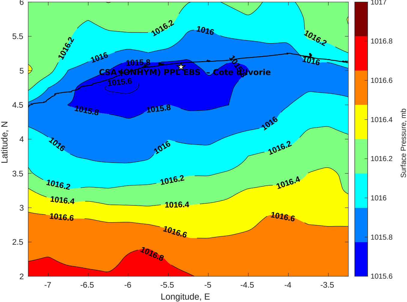
Surface Pressure (mb) for CSA (ONHYM) PPL EBS - Cote d'Ivoire at 28-Jul-2025 00:00:00
