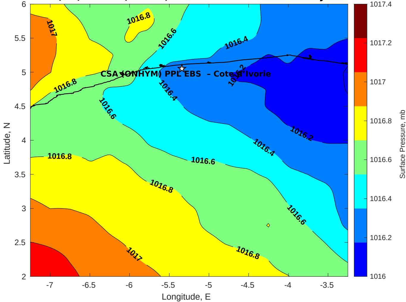
Surface Pressure (mb) for CSA (ONHYM) PPL EBS - Cote d'Ivoire at 29-Jul-2025 00:00:00
