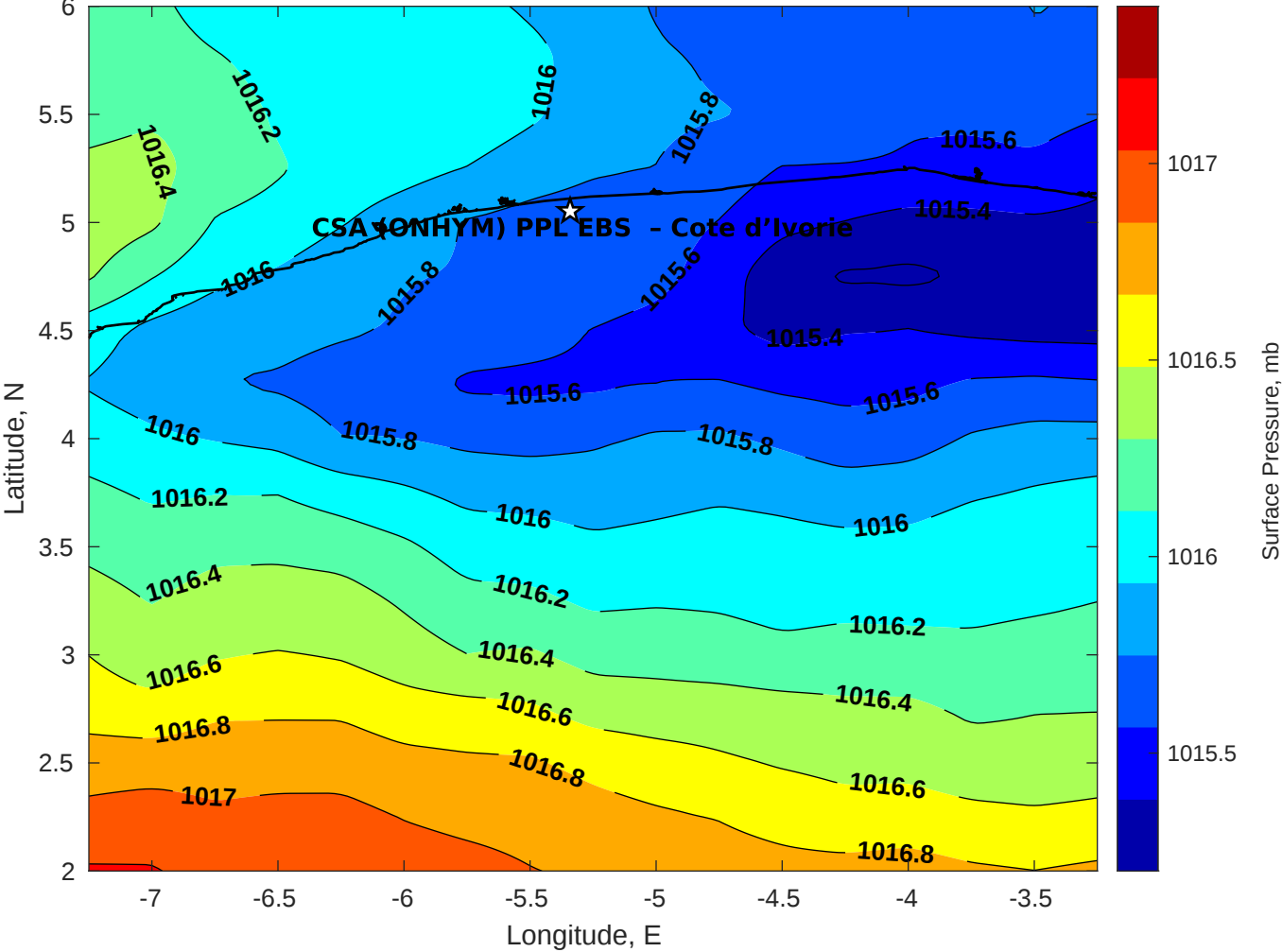
Surface Pressure (mb) for CSA (ONHYM) PPL EBS - Cote d'Ivoire at 30-Jul-2025 00:00:00
