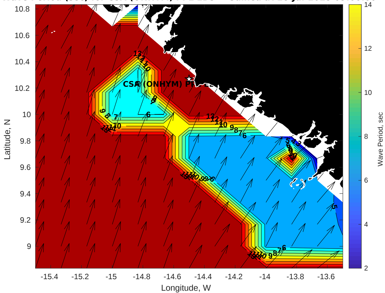
Wave Period (sec) for CSA (ONHYM) PPL EBS - Guinea at 28-Jul-2025 09:00:00
