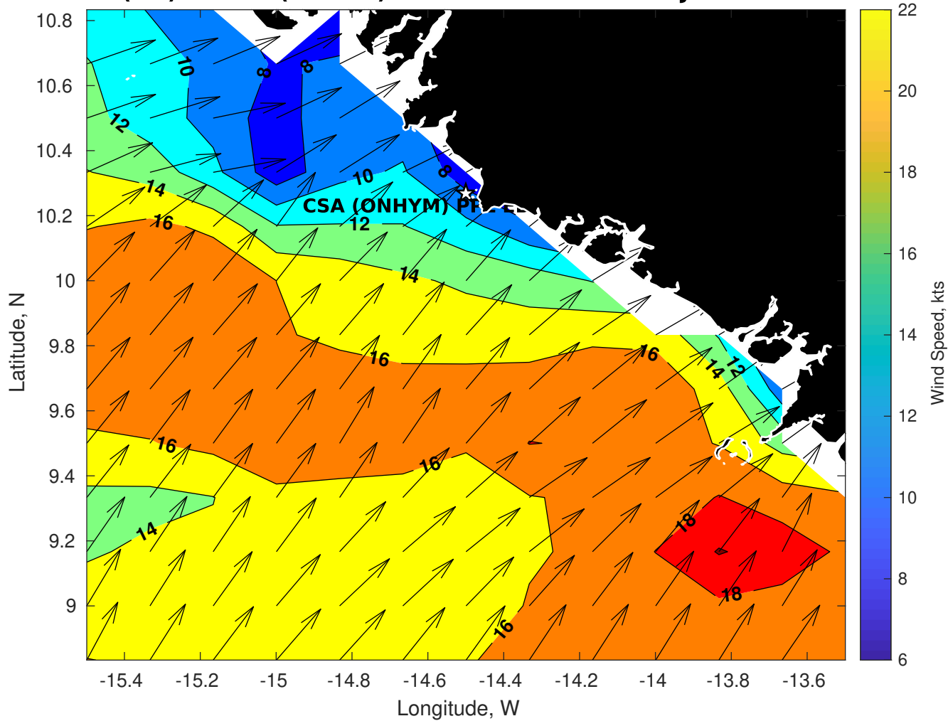
Winds (kts) for CSA (ONHYM) PPL EBS - Guinea at 28-Jul-2025 09:00:00
