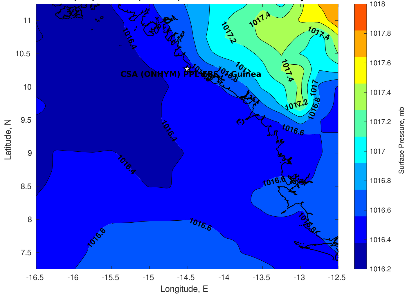
Surface Pressure (mb) for CSA (ONHYM) PPL EBS - Guinea at 30-Jul-2025 00:00:00
