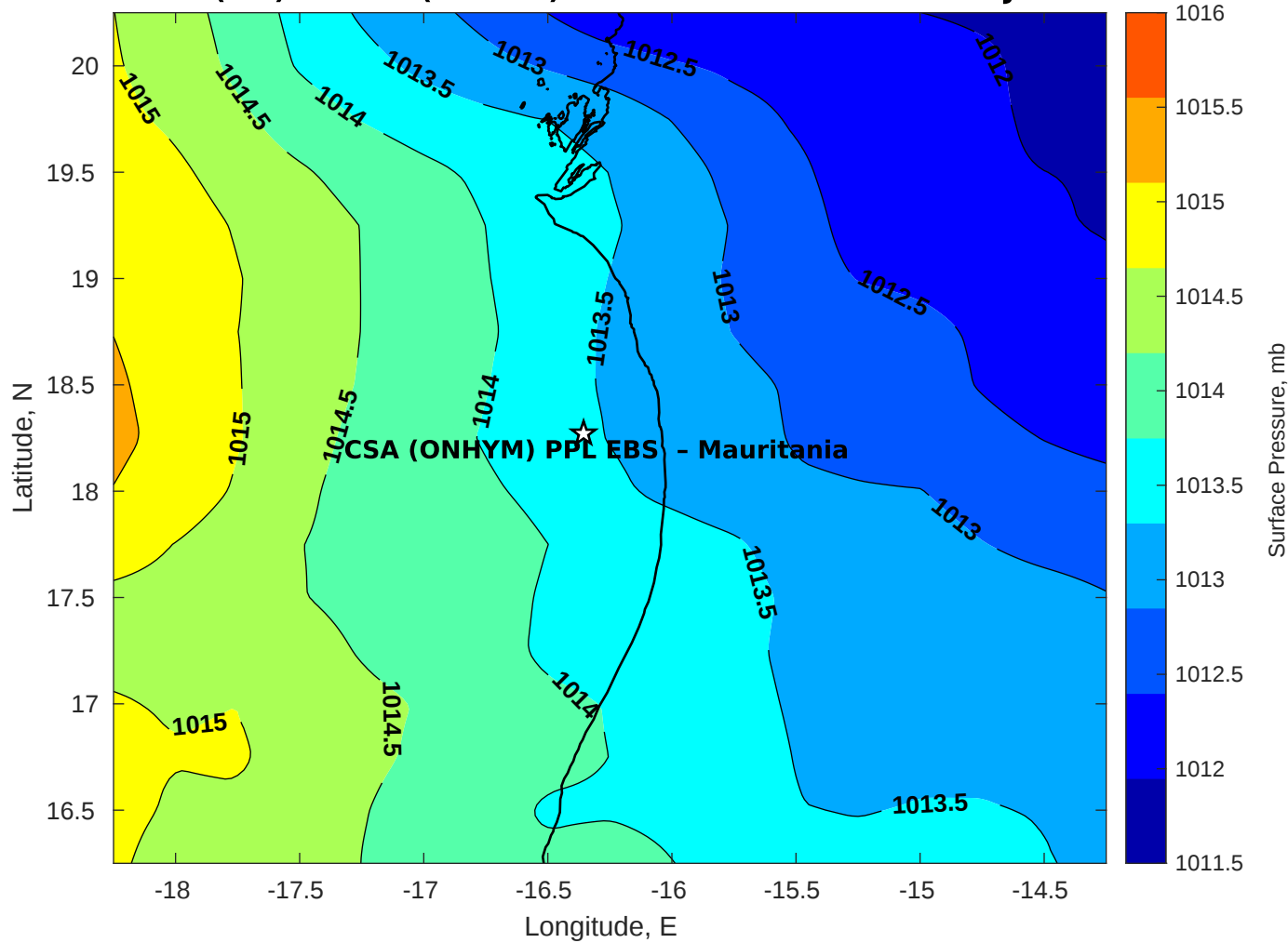
Surface Pressure (mb) for CSA (ONHYM) PPL EBS - Mauritania at 28-Jul-2025 00:00:00
