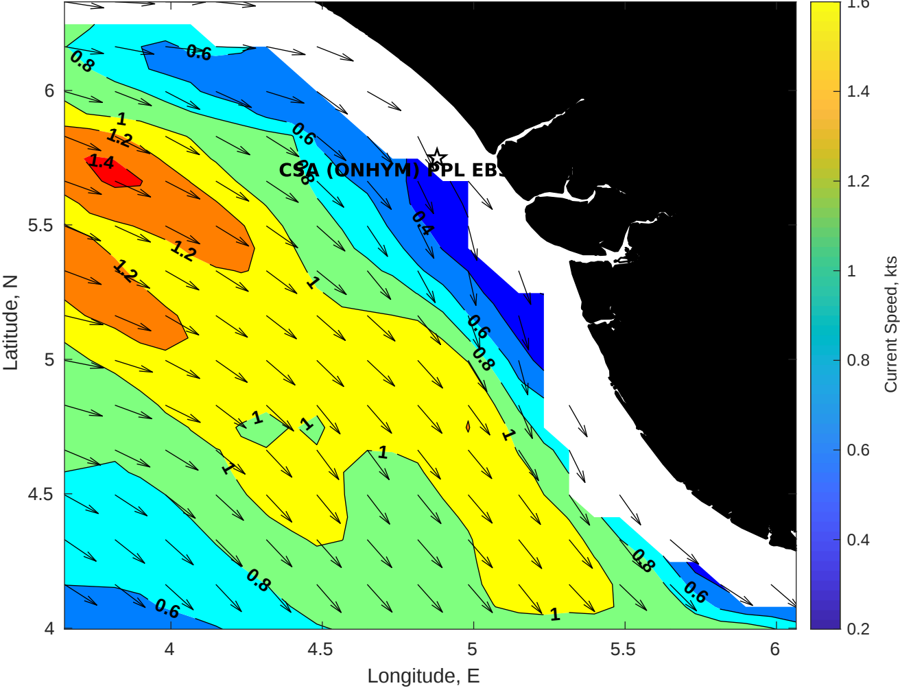
Surface Currents for CSA (ONHYM) PPL EBS - Nigeria at 25-Jul-2025 00:00:00
