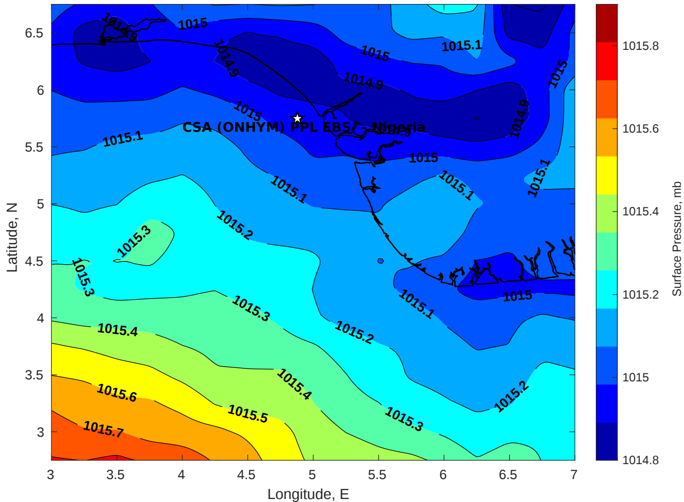
Surface Pressure (mb) for CSA (ONHYM) PPL EBS - Nigeria at 30-Jul-2025 00:00:00
