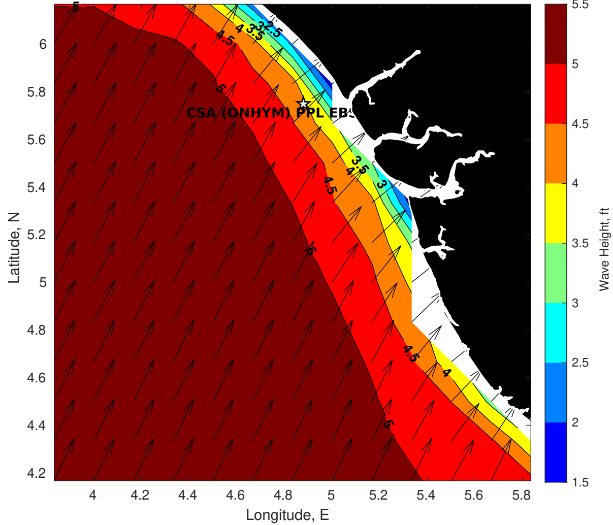
Wave Height (ft) for CSA (ONHYM) PPL EBS - Nigeria at 28-Jul-2025 09:00:00
