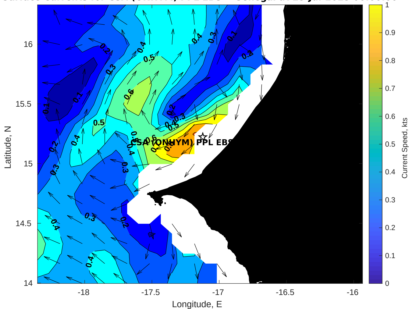
Surface Currents for CSA (ONHYM) PPL EBS - Senegal at 25-Jul-2025 00:00:00
