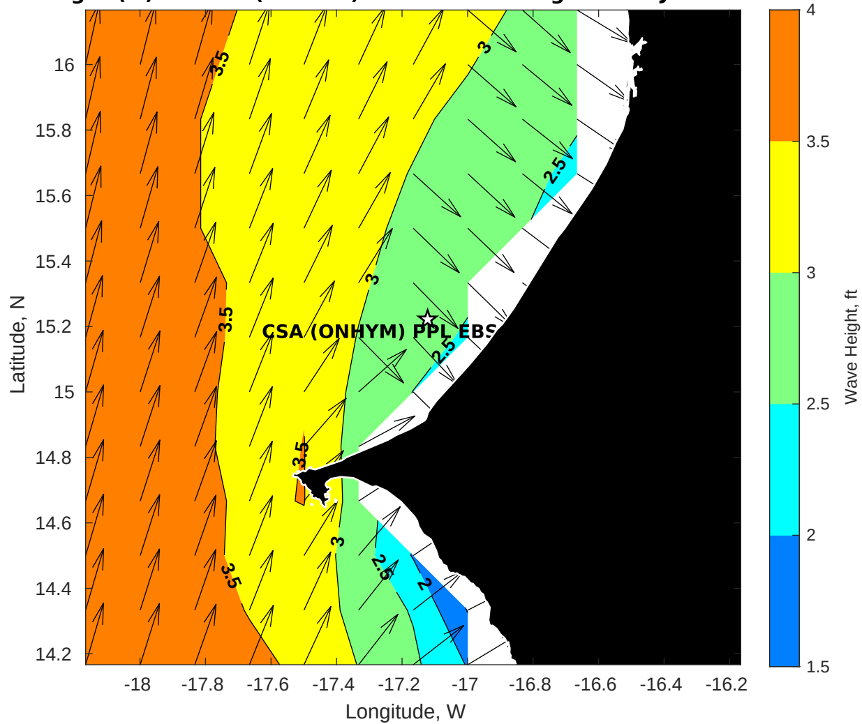
Wave Height (ft) for CSA (ONHYM) PPL EBS - Senegal at 28-Jul-2025 09:00:00
