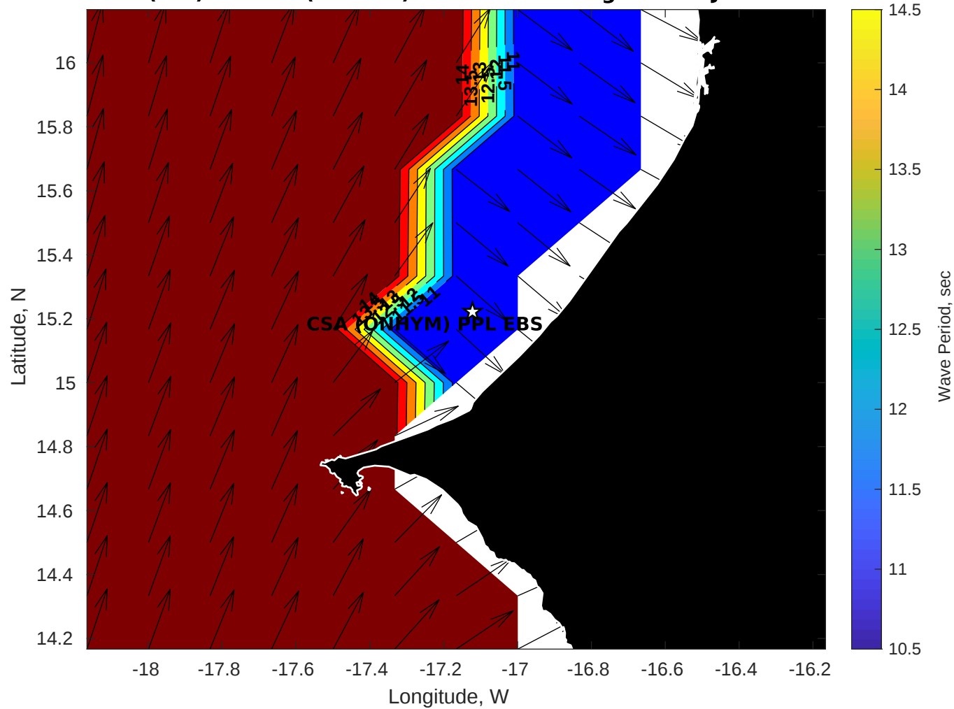
Wave Period (sec) for CSA (ONHYM) PPL EBS - Senegal at 28-Jul-2025 09:00:00
