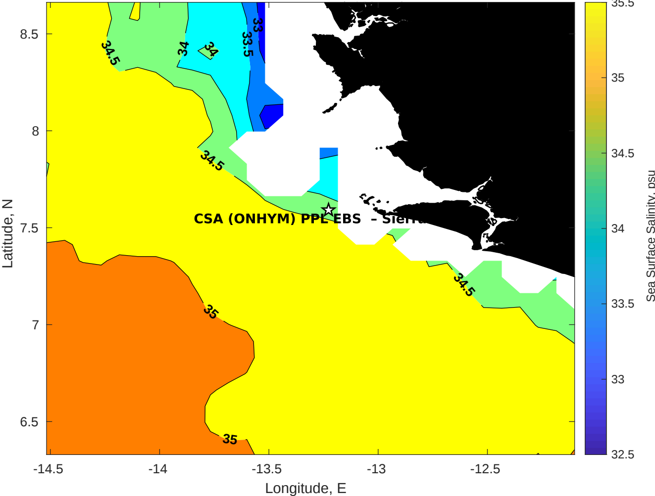
Surface Salinity for CSA (ONHYM) PPL EBS - Sierra Leone at 25-Jul-2025 00:00:00
