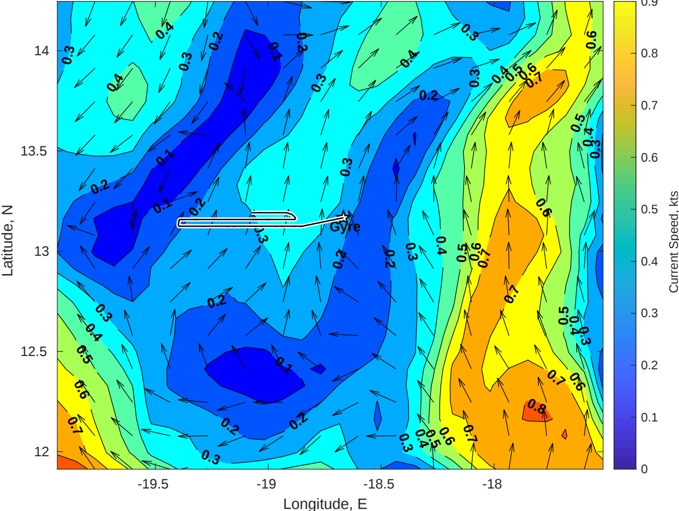
Surface Currents for Gyre at 28-Jul-2025 00:00:00
