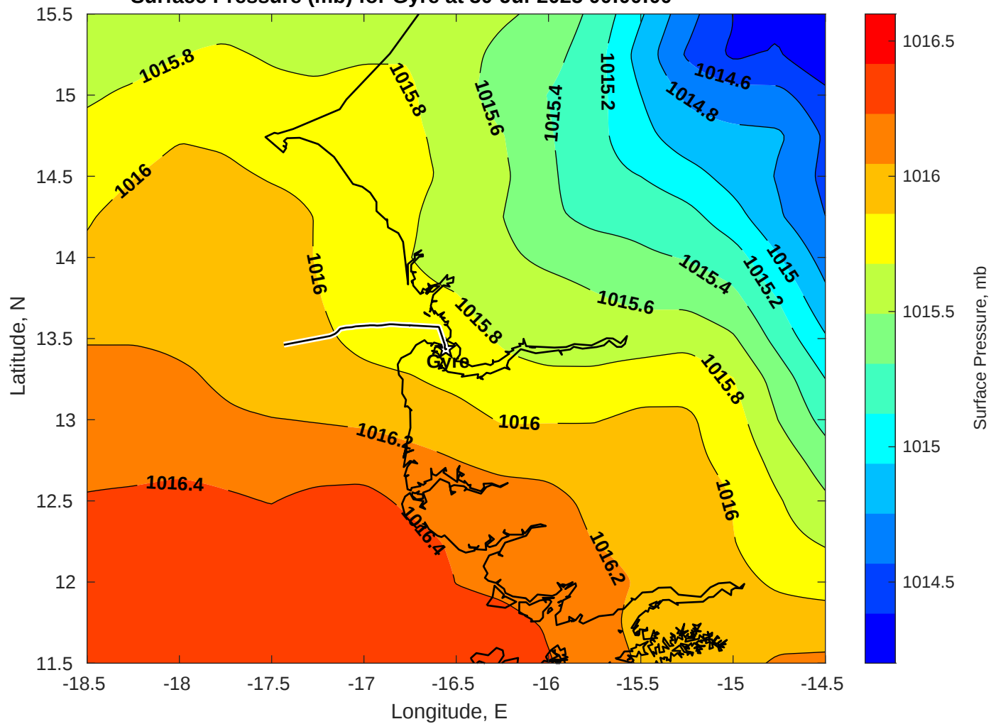
Surface Pressure (mb) for Gyre at 30-Jul-2025 00:00:00
