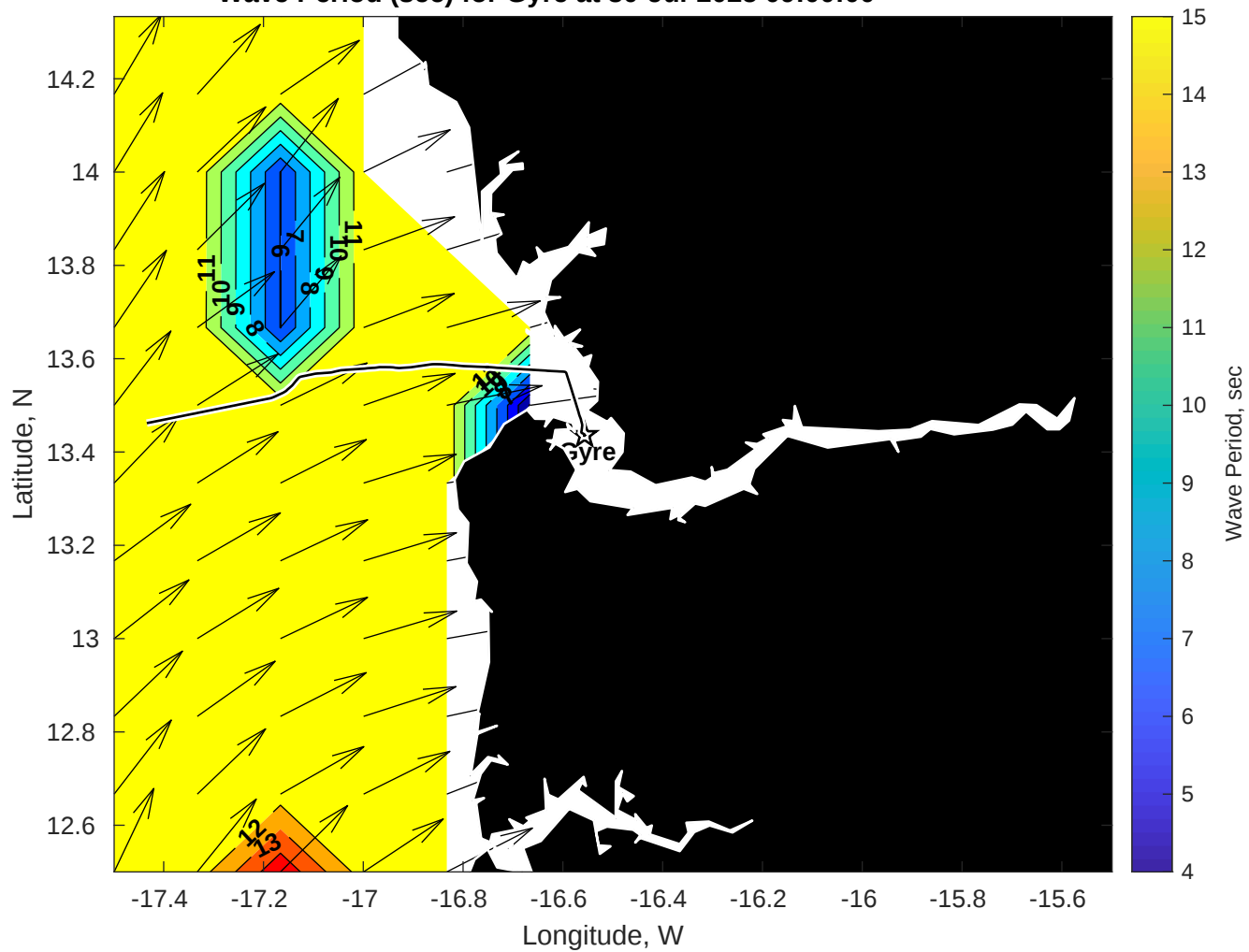
Wave Period (sec) for Gyre at 30-Jul-2025 09:00:00
