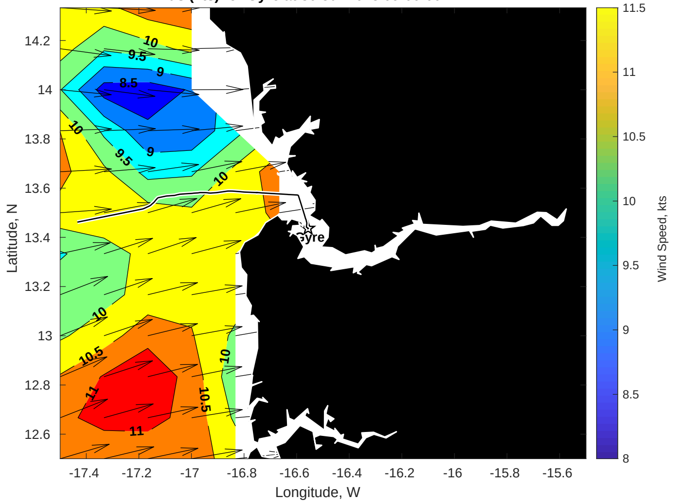
Winds (kts) for Gyre at 30-Jul-2025 09:00:00
