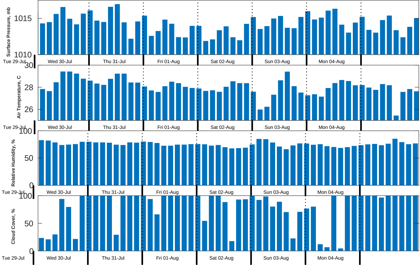
Met Forecast for Gyre from 29-Jul-2025 23:00:00 to 05-Aug-2025 23:00:00
