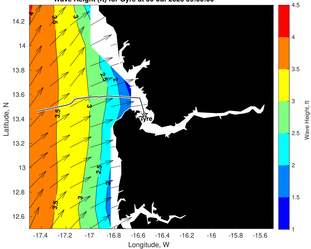
Wave Height (ft) for Gyre at 30-Jul-2025 09:00:00
