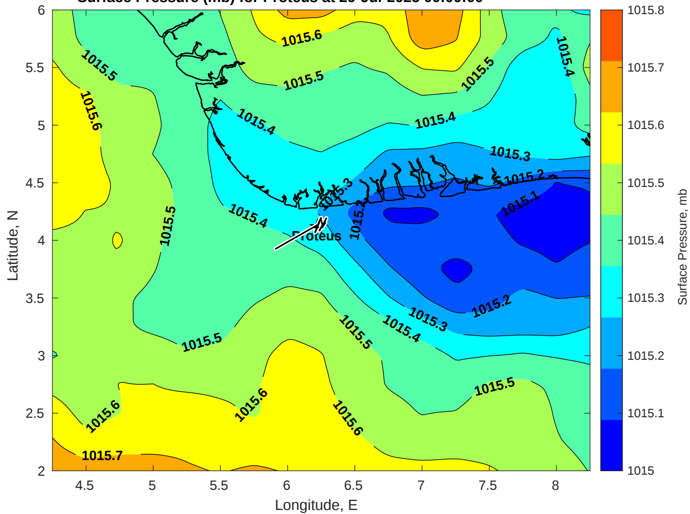
Surface Pressure (mb) for Proteus at 29-Jul-2025 00:00:00
