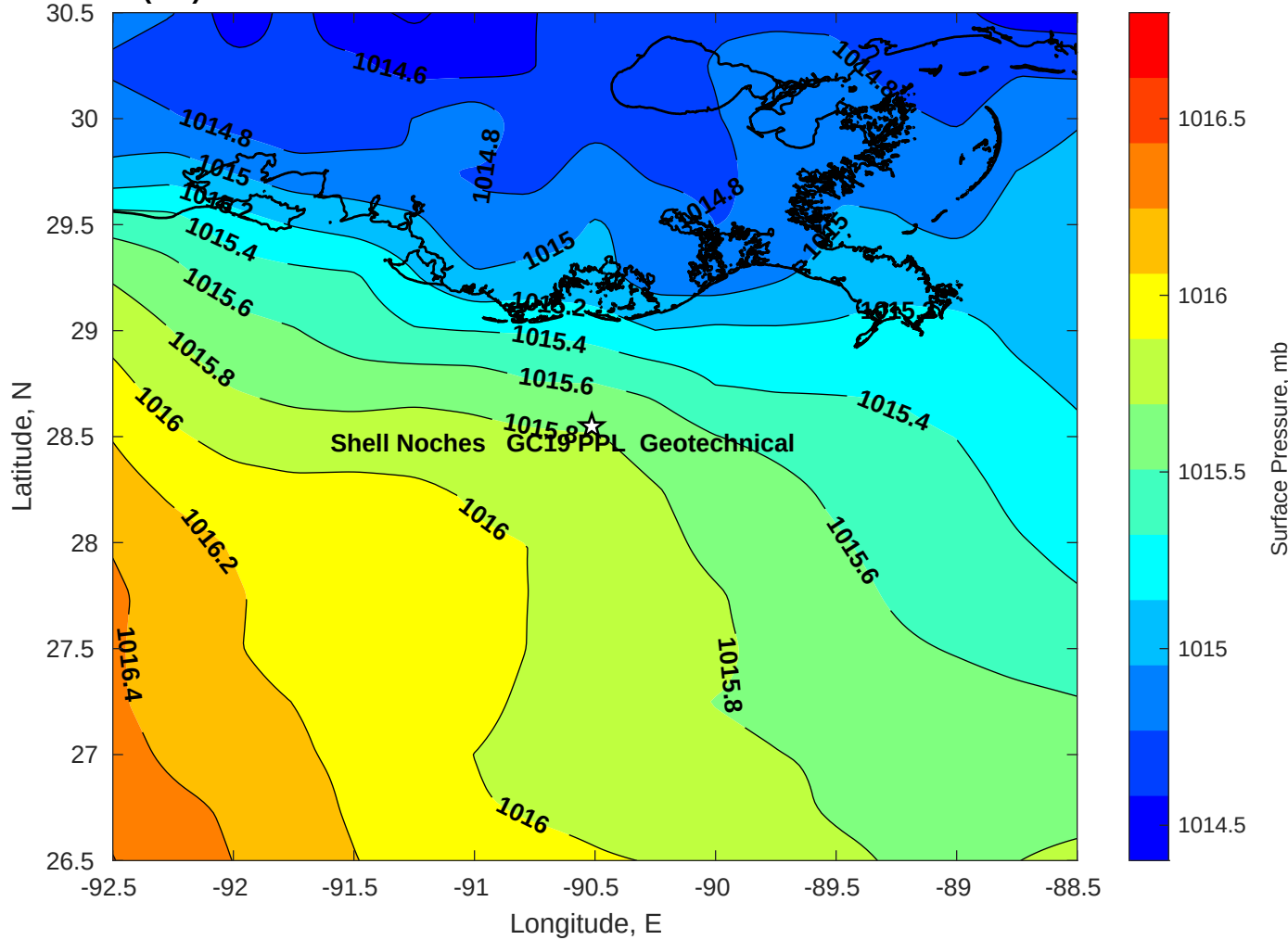
Surface Pressure (mb) for Shell Noches GC19 PPL Geotechnical at 30-Jul-2025 00:00:00
