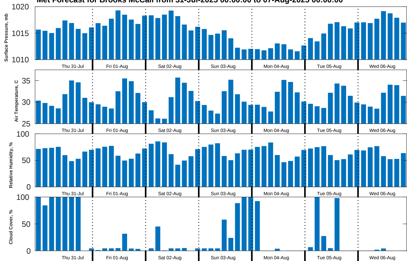
Met Forecast for Brooks McCall from 31-Jul-2025 00:00:00 to 07-Aug-2025 00:00:00
