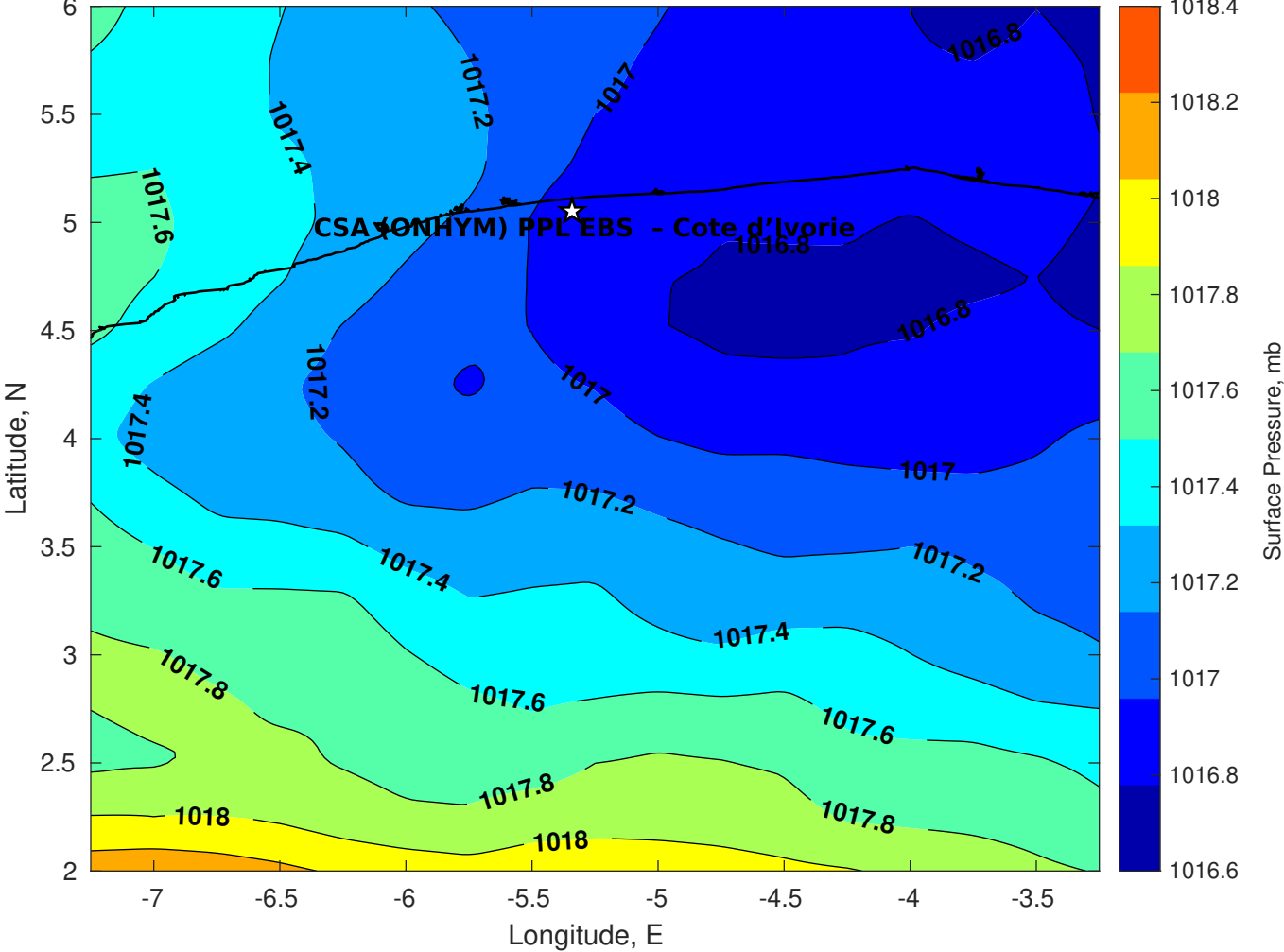
Surface Pressure (mb) for CSA (ONHYM) PPL EBS - Cote d'Ivoire at 31-Jul-2025 00:00:00
