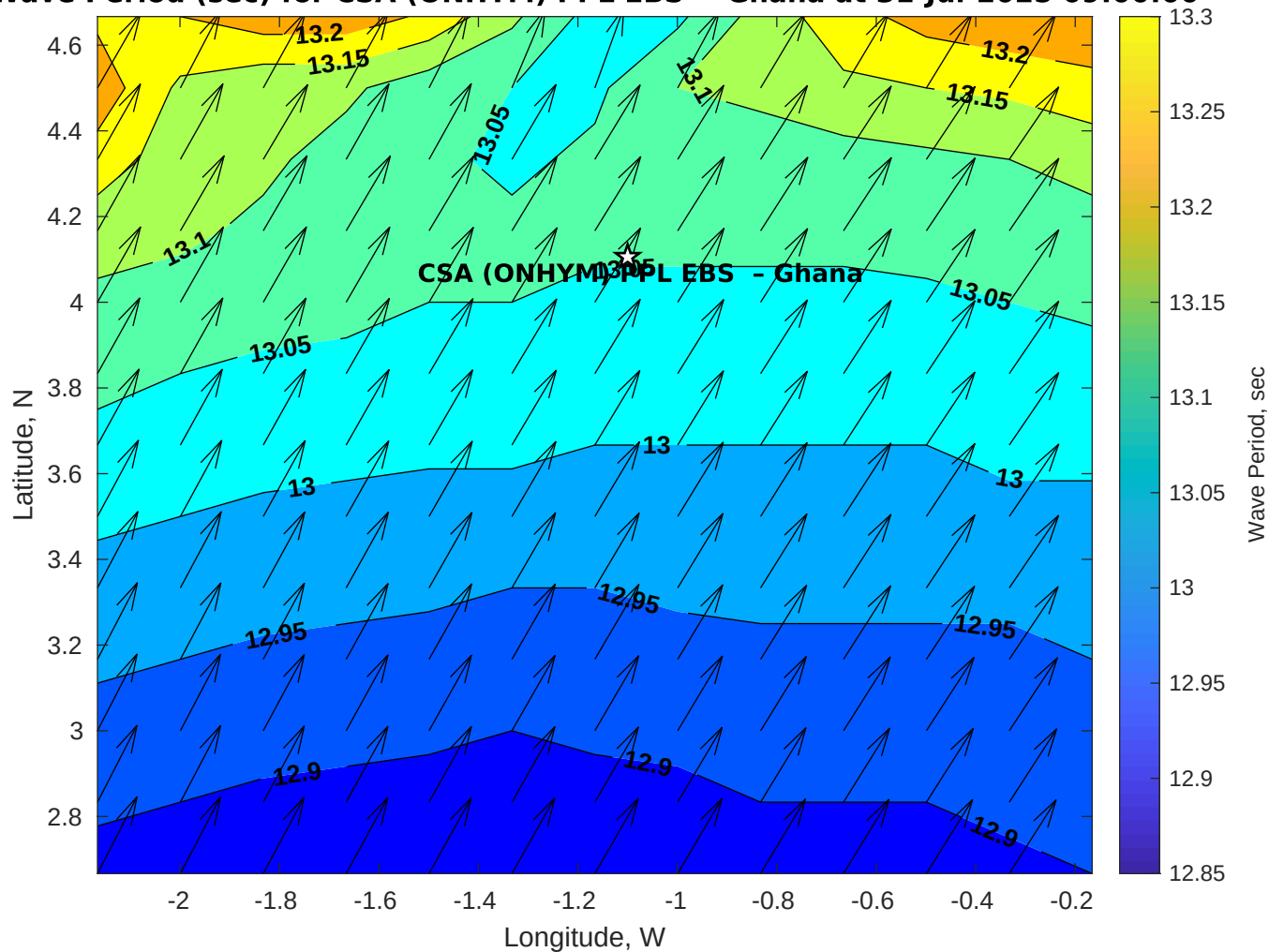
Wave Period (sec) for CSA (ONHYM) PPL EBS - Ghana at 31-Jul-2025 09:00:00
