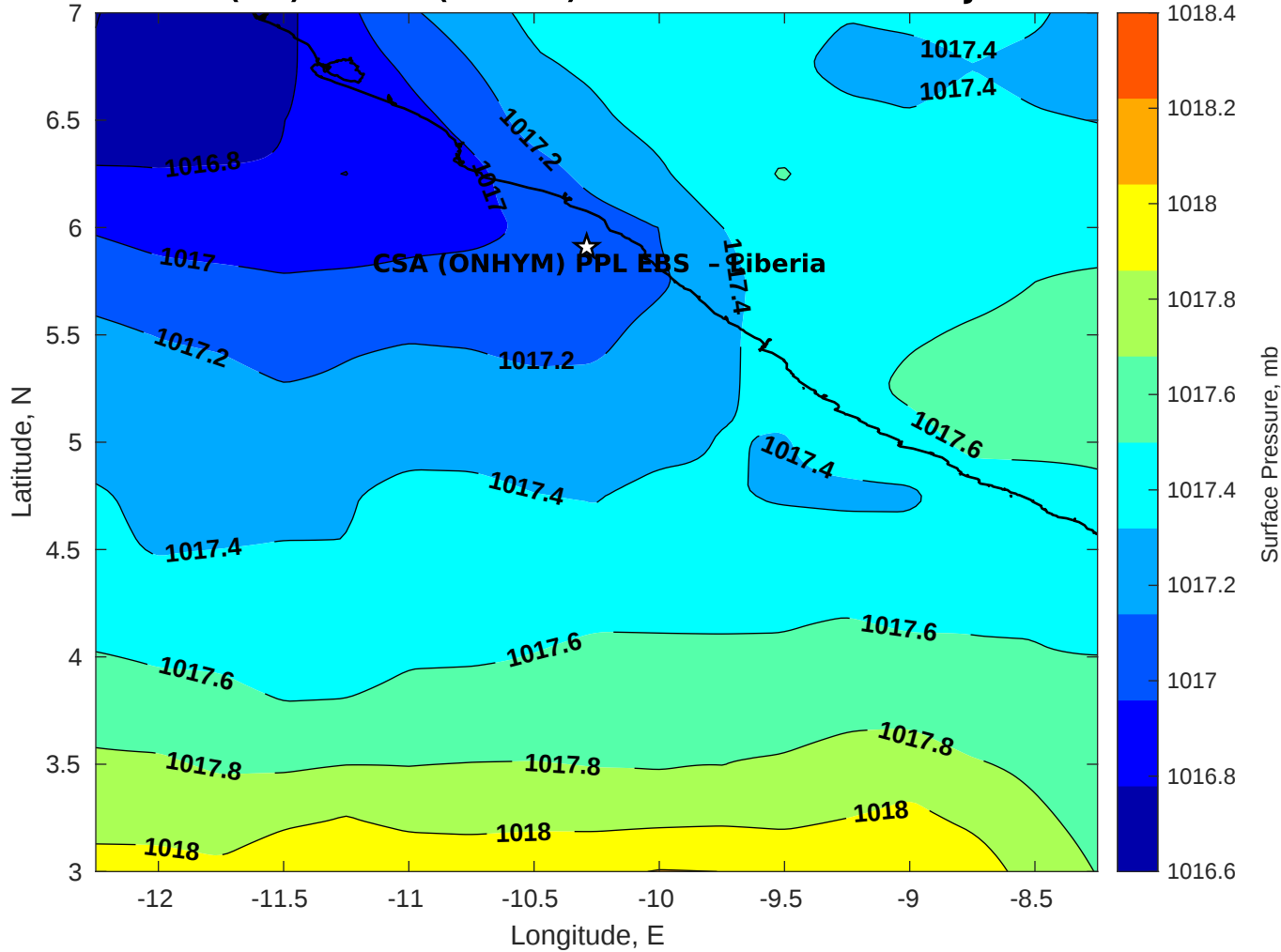
Surface Pressure (mb) for CSA (ONHYM) PPL EBS - Liberia at 31-Jul-2025 00:00:00
