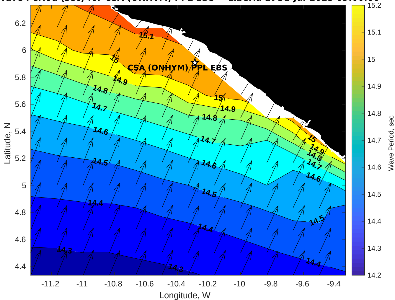
Wave Period (sec) for CSA (ONHYM) PPL EBS - Liberia at 31-Jul-2025 09:00:00
