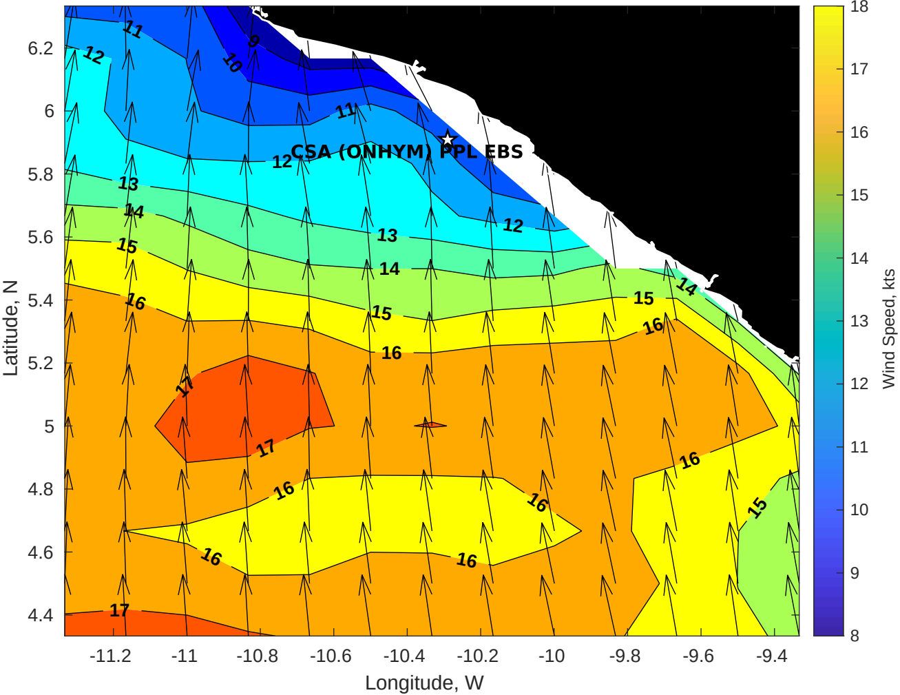
Winds (kts) for CSA (ONHYM) PPL EBS - Liberia at 31-Jul-2025 09:00:00
