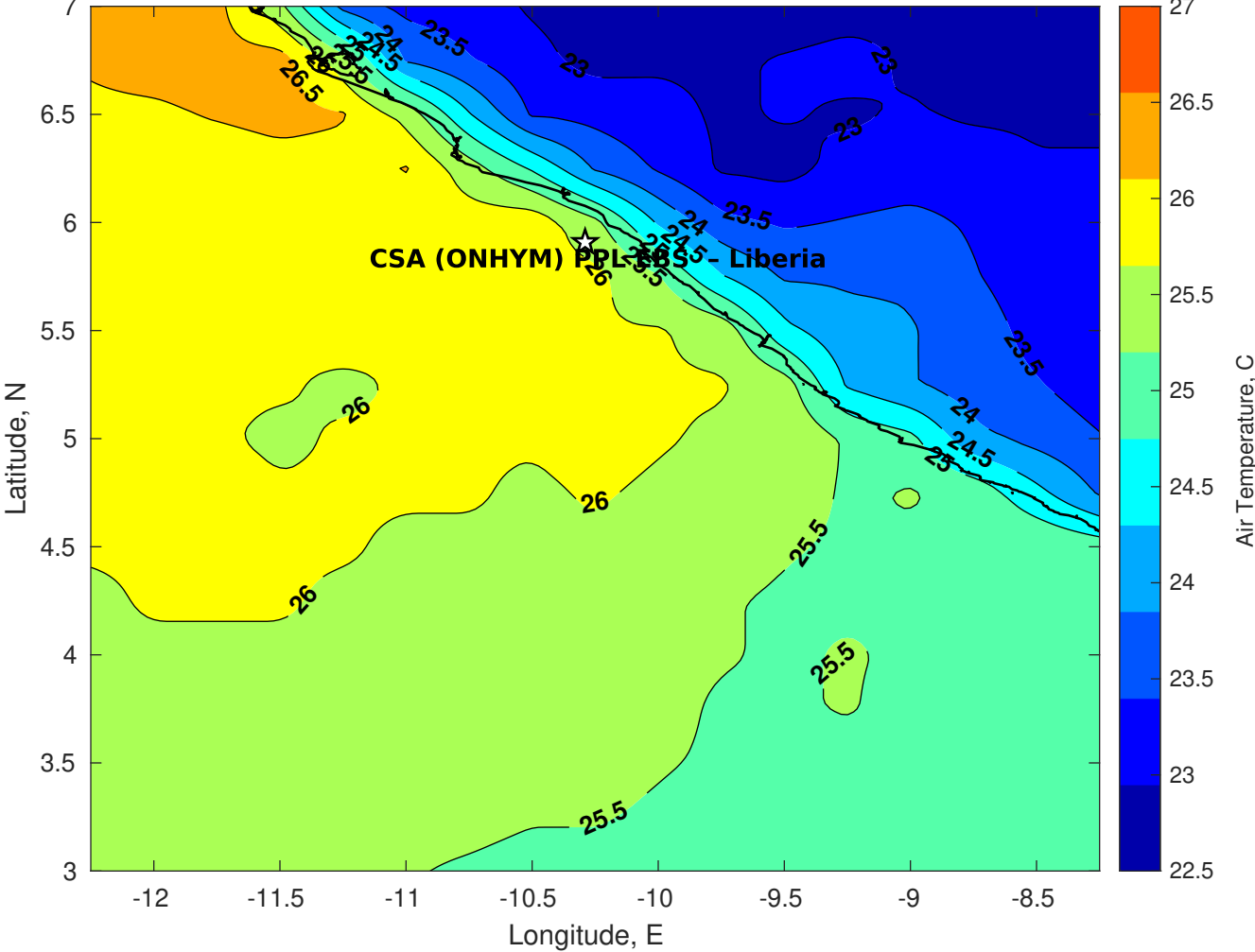
Air Temperature (C) for CSA (ONHYM) PPL EBS - Liberia at 31-Jul-2025
