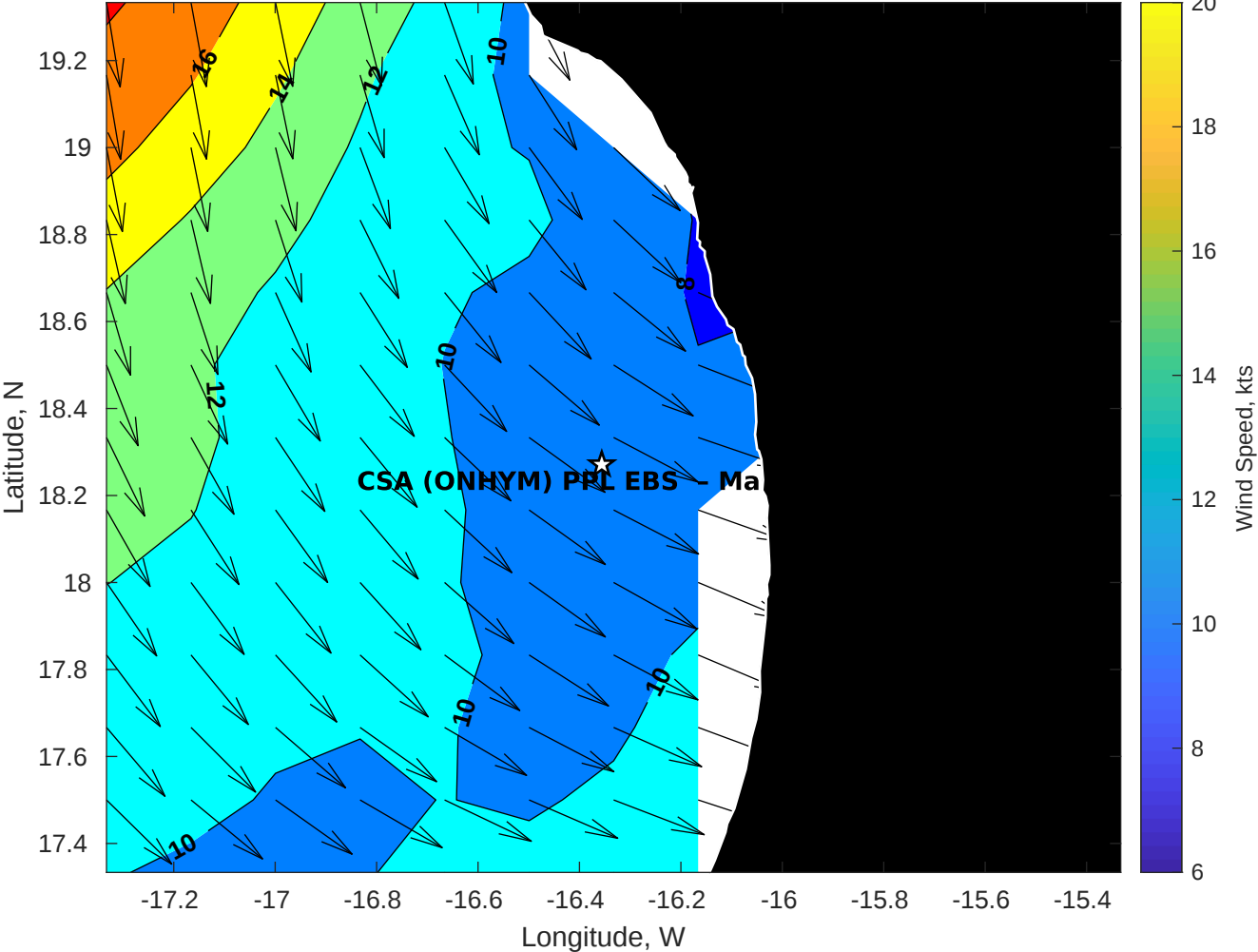
Winds (kts) for CSA (ONHYM) PPL EBS - Mauritania at 31-Jul-2025 09:00:00
