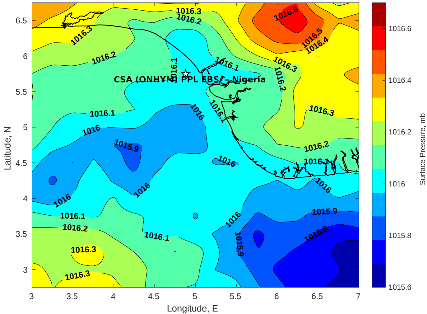
Surface Pressure (mb) for CSA (ONHYM) PPL EBS - Nigeria at 01-Aug-2025 00:00:00
