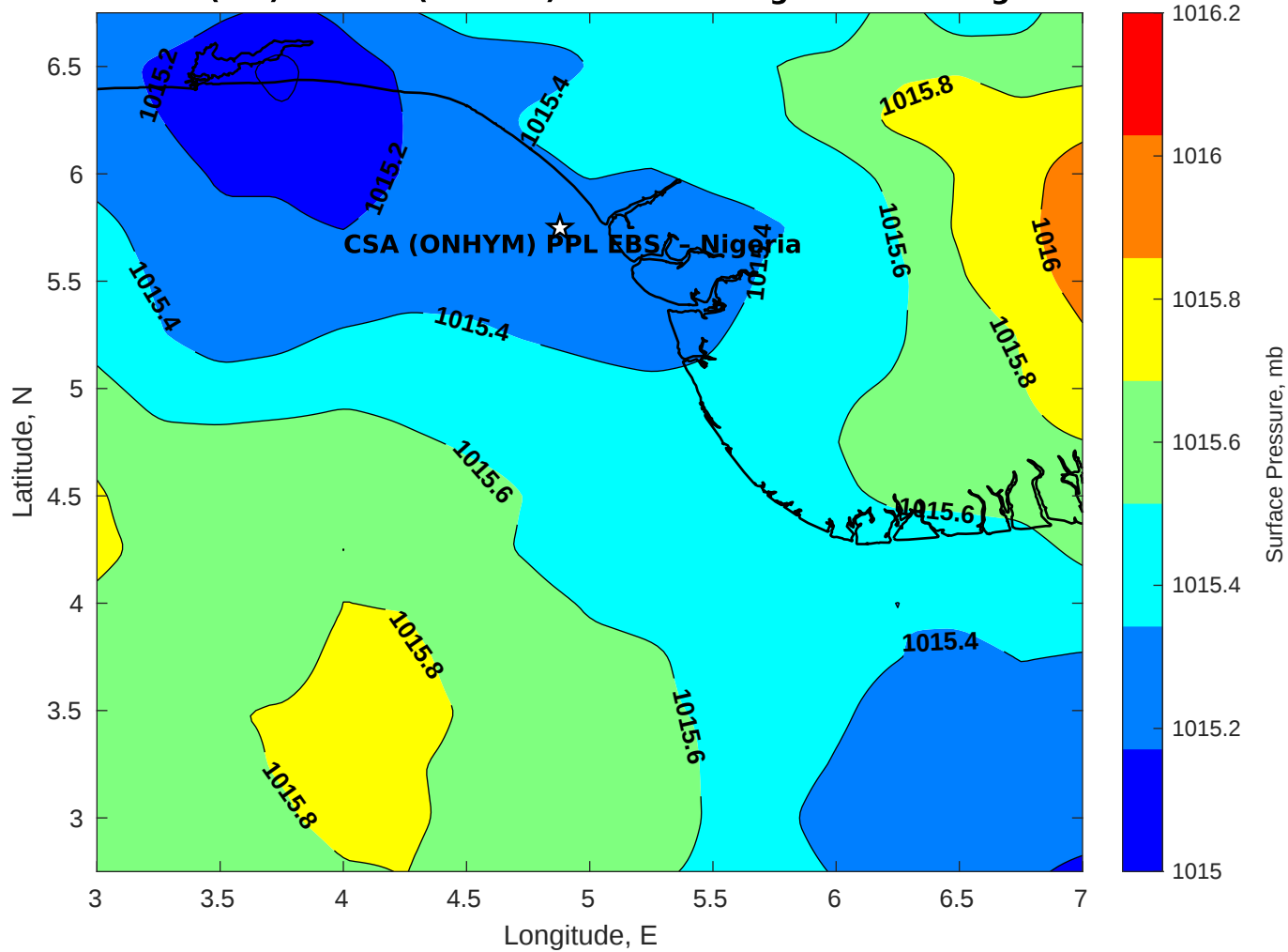
Surface Pressure (mb) for CSA (ONHYM) PPL EBS - Nigeria at 02-Aug-2025 00:00:00
