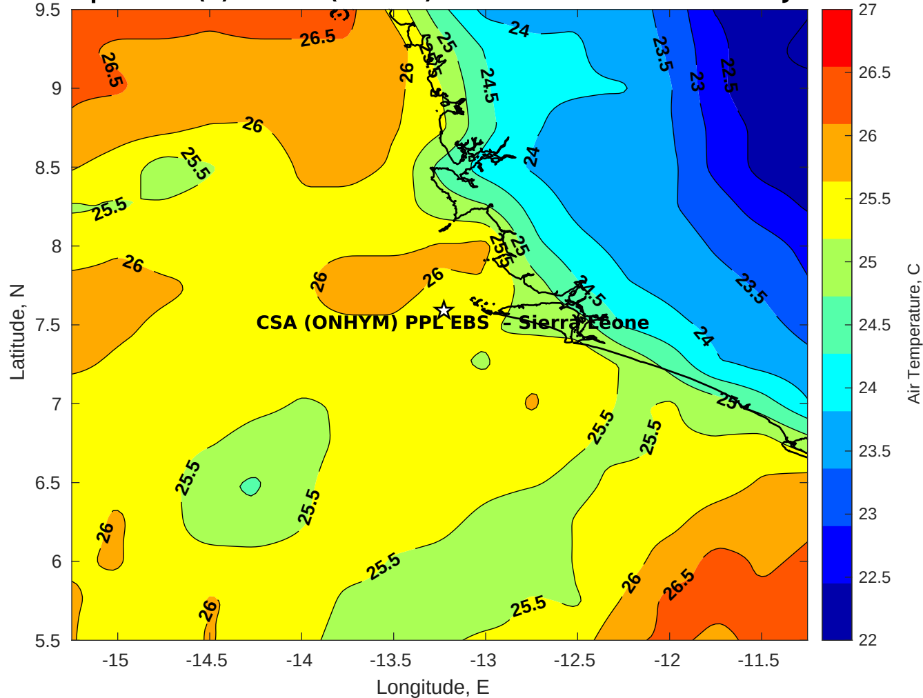
Air Temperature (C) for CSA (ONHYM) PPL EBS - Sierra Leone at 31-Jul-2025
