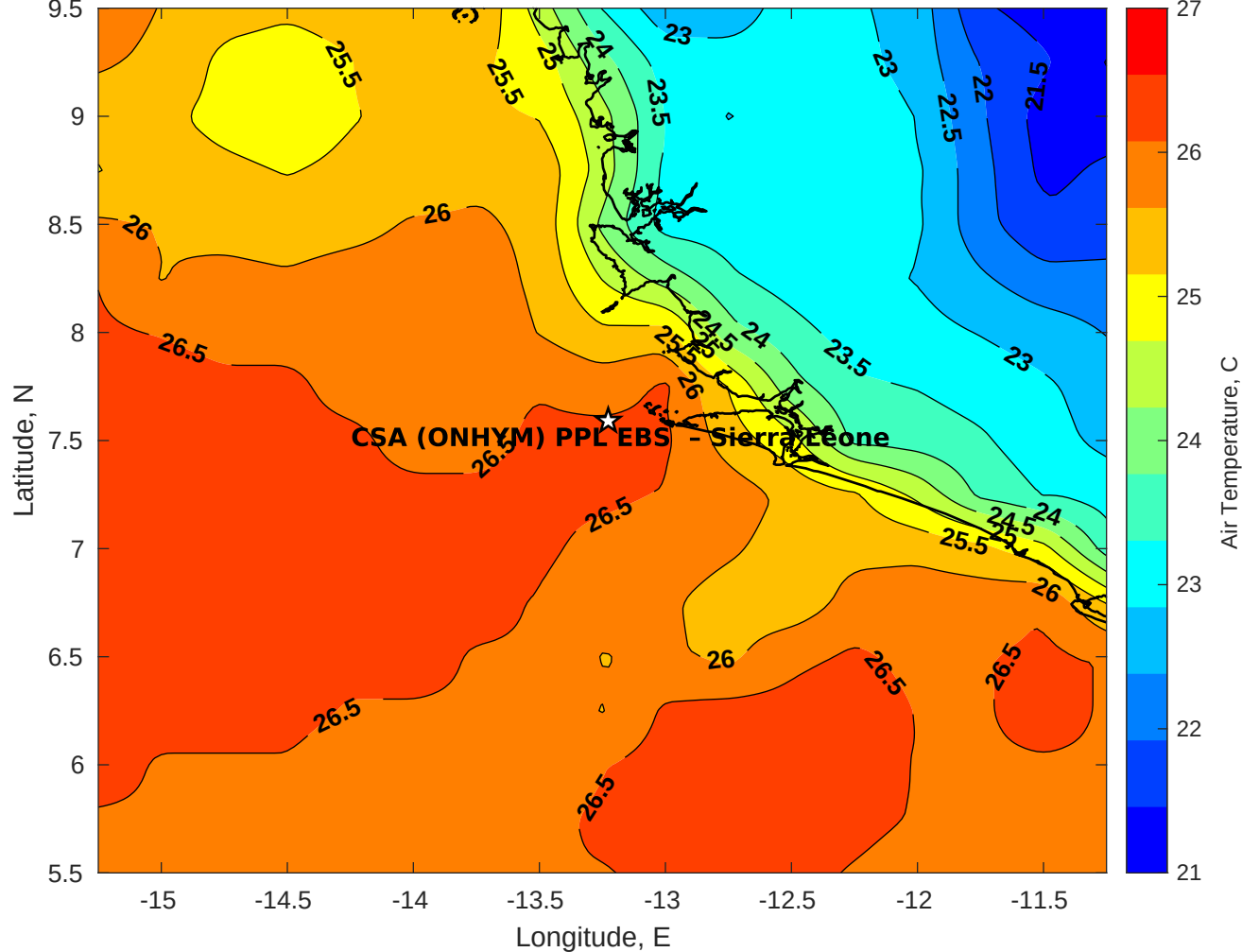
Air Temperature (C) for CSA (ONHYM) PPL EBS - Sierra Leone at 31-Jul-2025
