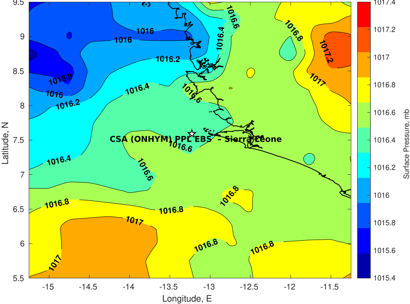
Surface Pressure (mb) for CSA (ONHYM) PPL EBS - Sierra Leone at 02-Aug-2025 00:00:00
