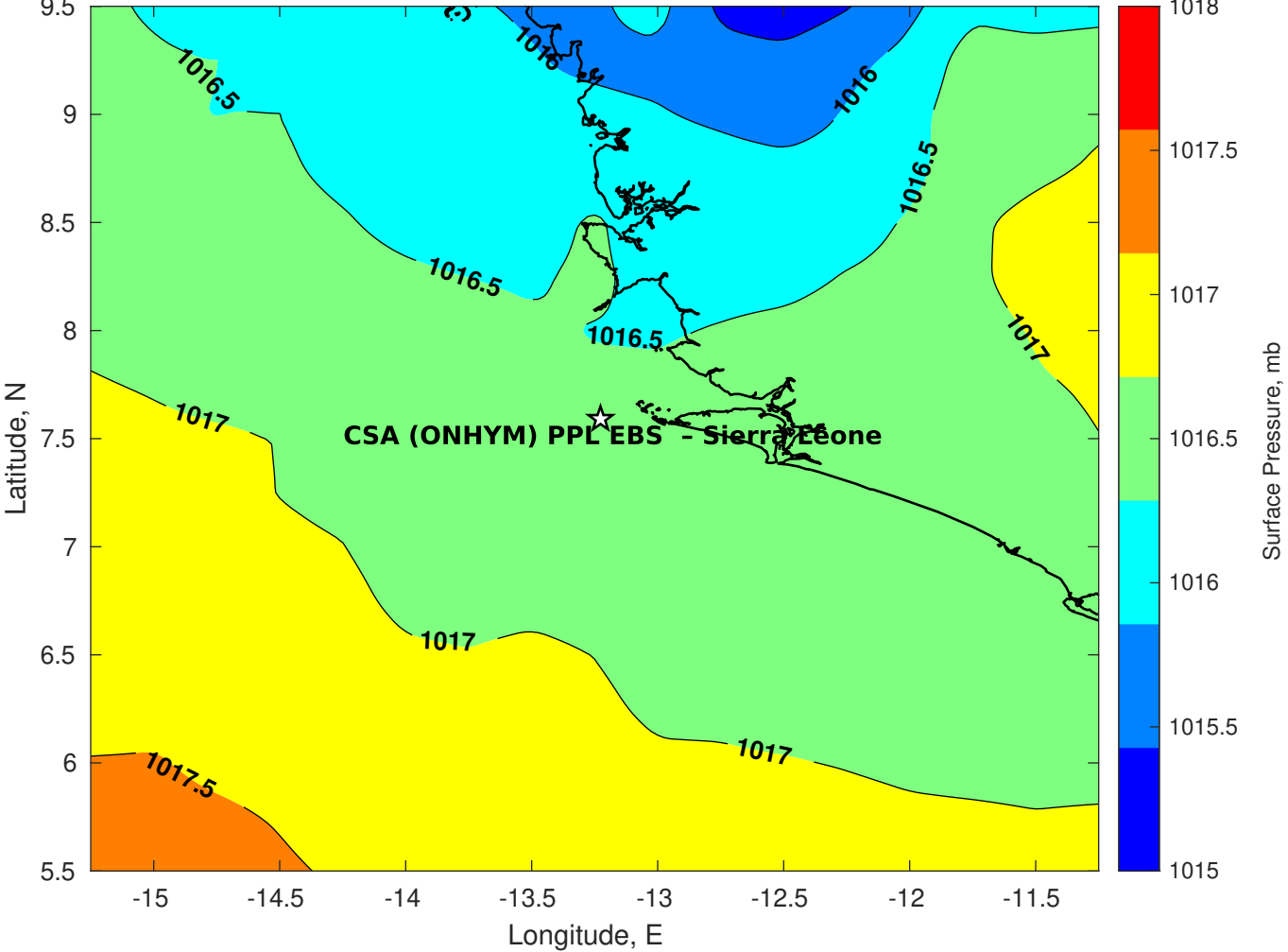
Surface Pressure (mb) for CSA (ONHYM) PPL EBS - Sierra Leone at 31-Jul-2025 00:00:00
