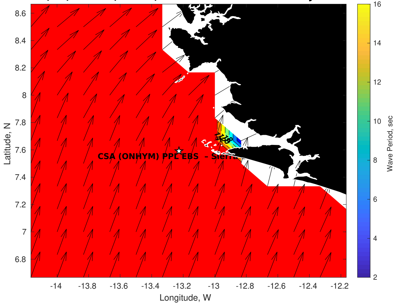
Wave Period (sec) for CSA (ONHYM) PPL EBS - Sierra Leone at 31-Jul-2025 09:00:00
