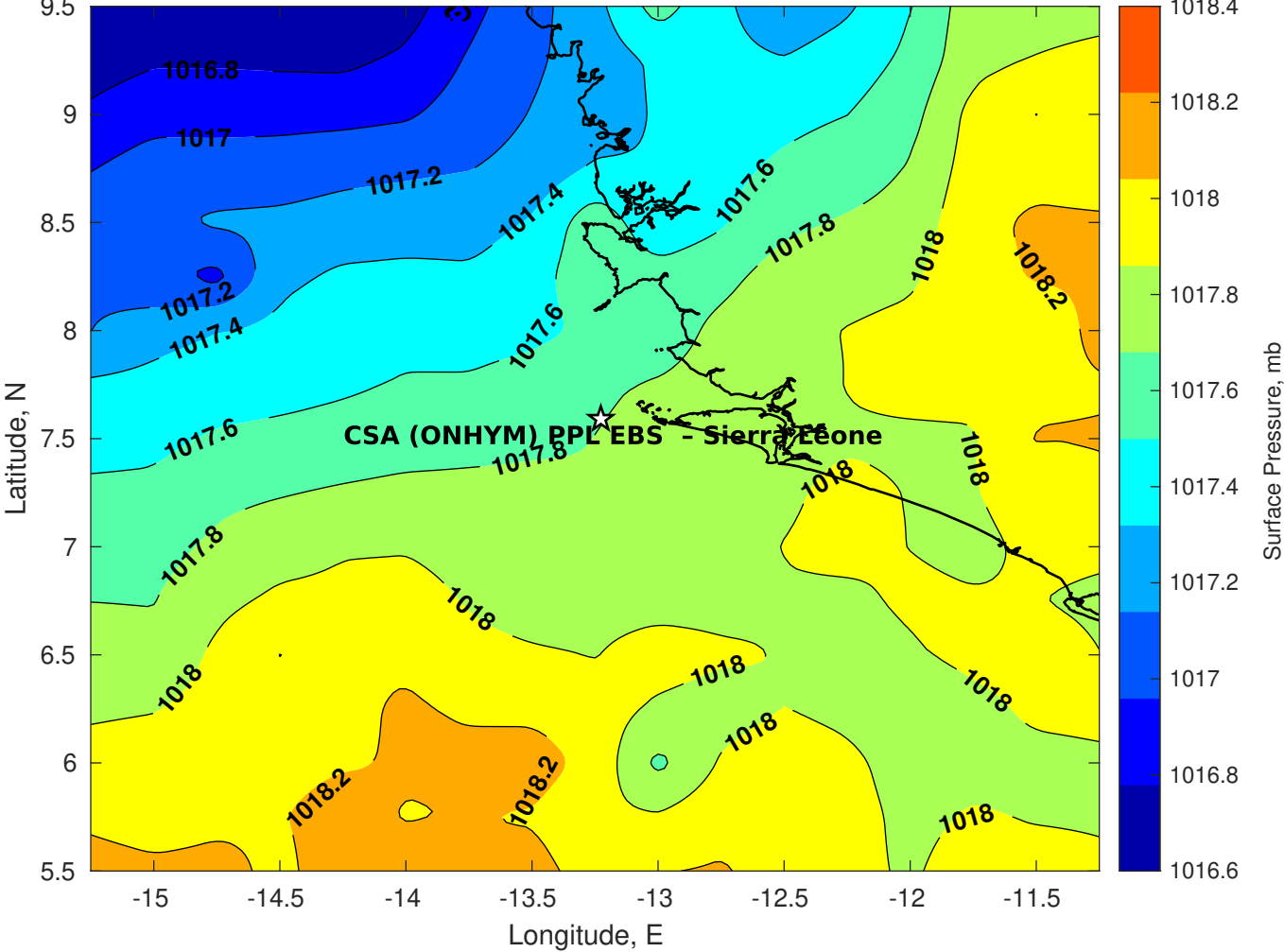
Surface Pressure (mb) for CSA (ONHYM) PPL EBS - Sierra Leone at 01-Aug-2025 00:00:00
