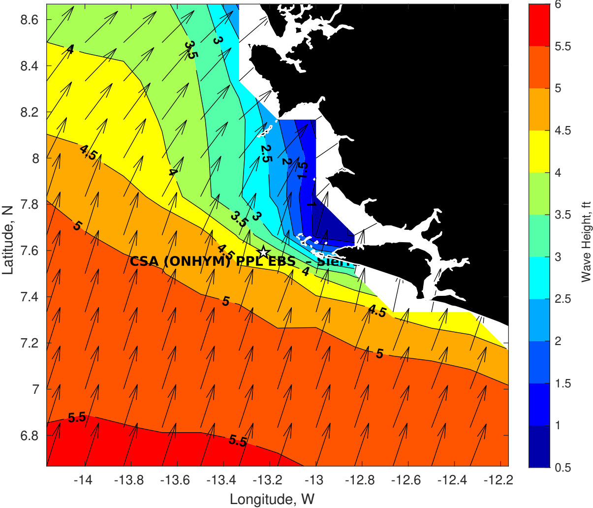
Wave Height (ft) for CSA (ONHYM) PPL EBS - Sierra Leone at 31-Jul-2025 09:00:00
