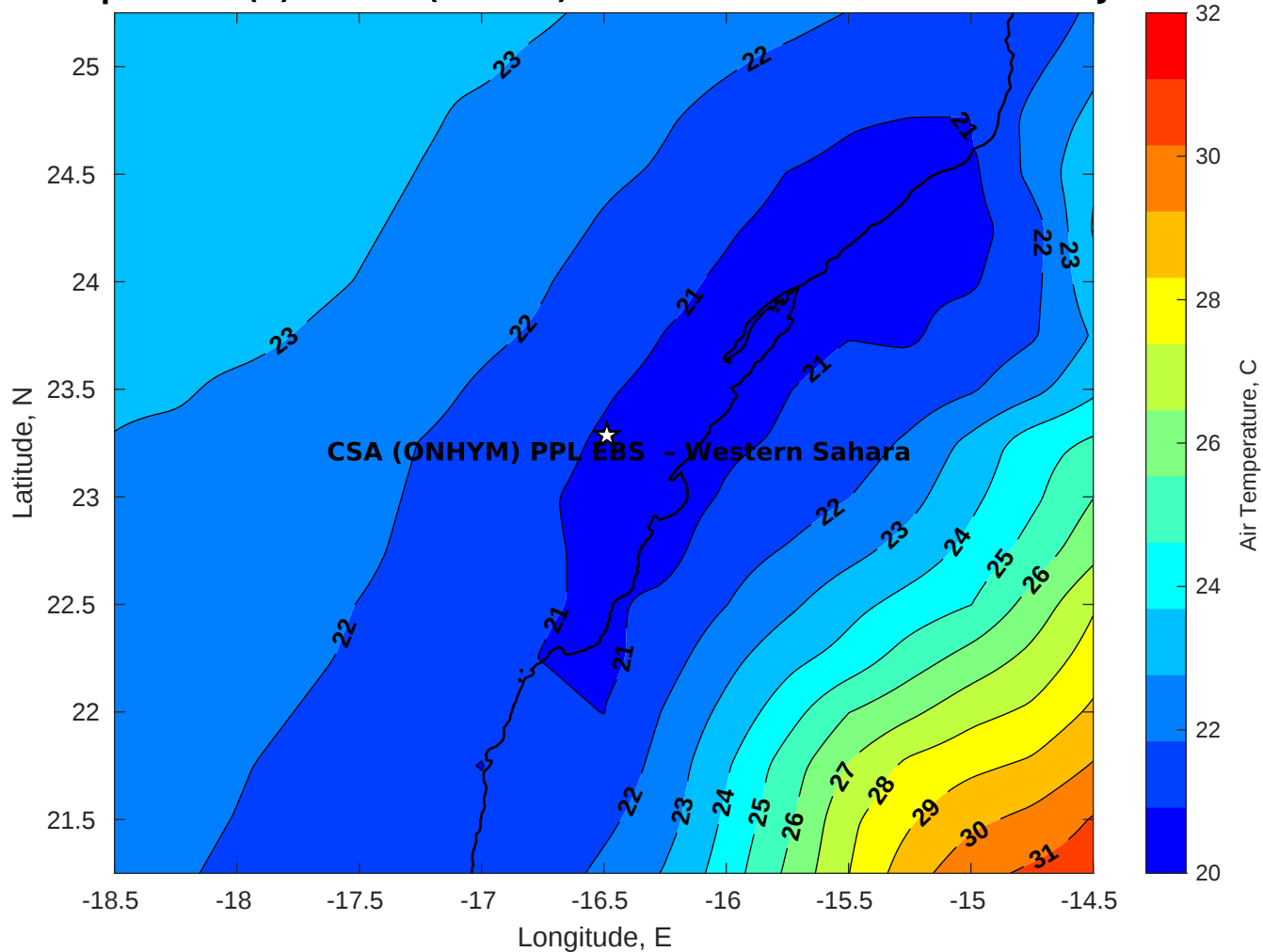
Air Temperature (C) for CSA (ONHYM) PPL EBS - Western Sahara at 31-Jul-2025
