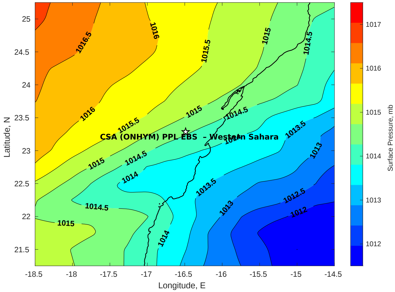
Surface Pressure (mb) for CSA (ONHYM) PPL EBS - Western Sahara at 31-Jul-2025 00:00:00
