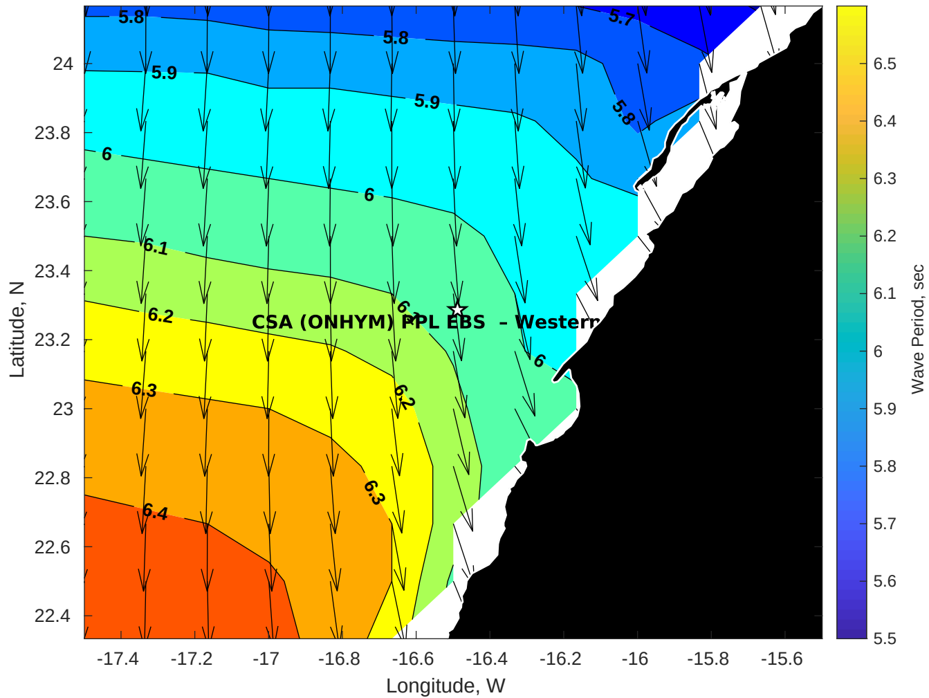
Wave Period (sec) for CSA (ONHYM) PPL EBS - Western Sahara at 31-Jul-2025 09:00:00
